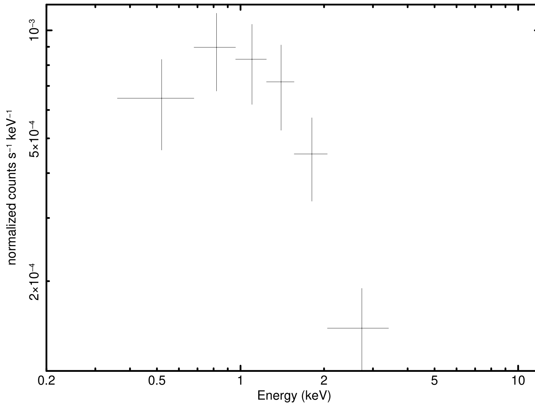
Source 27 minus background (P0931790101M2S002SRSPEC001B)
