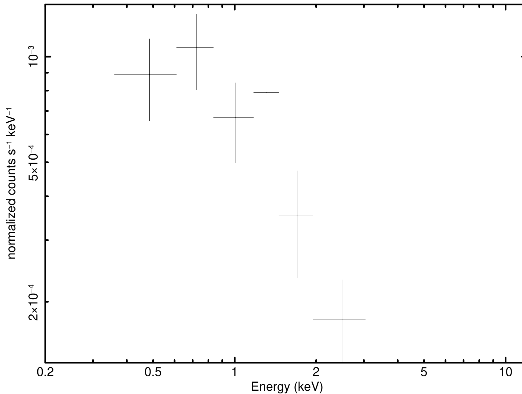
Source 29 minus background (P0931790101M2S002SRSPEC001D)
