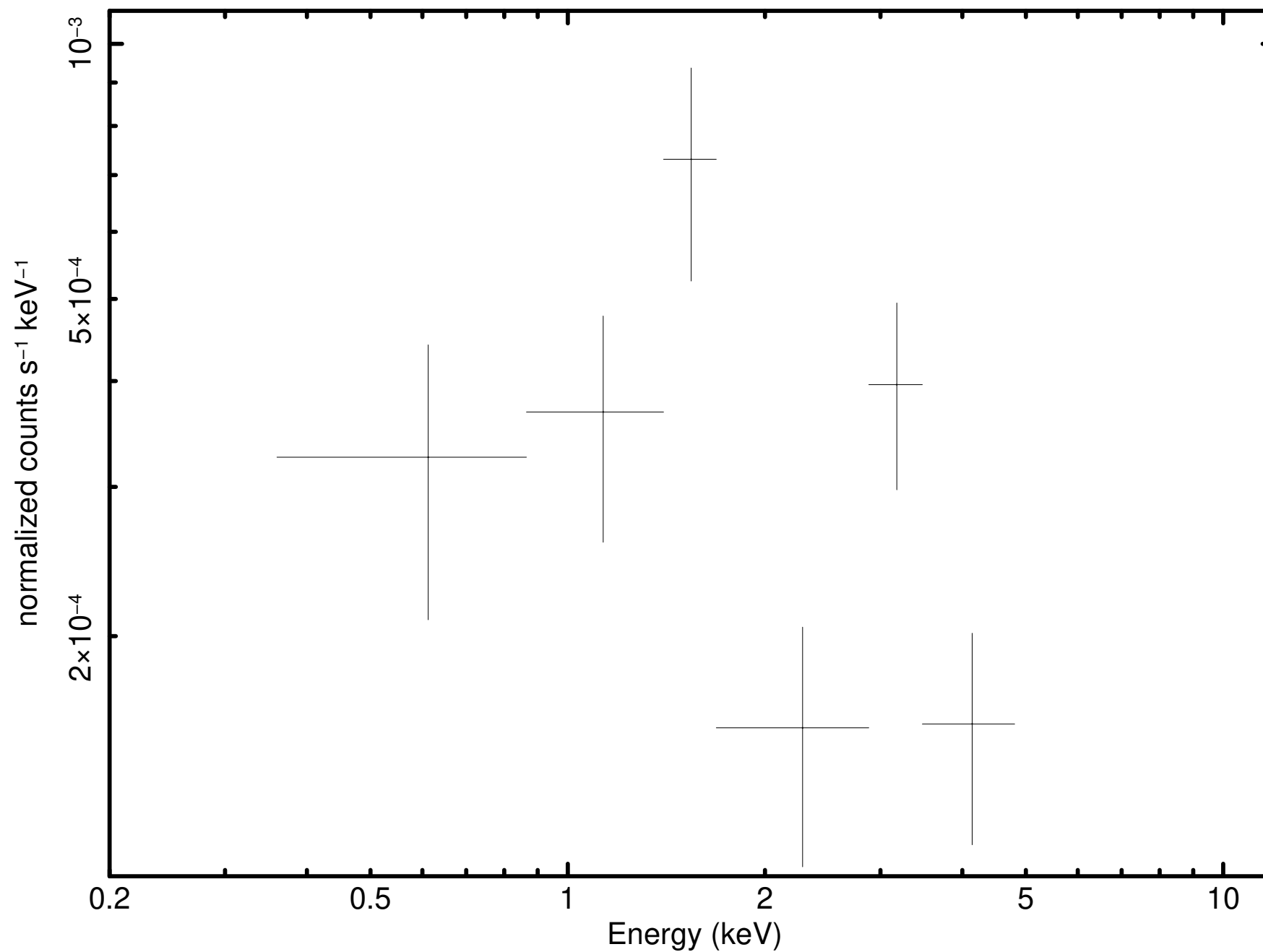
Source 32 minus background (P0931790101M2S002SRSPEC0020)
