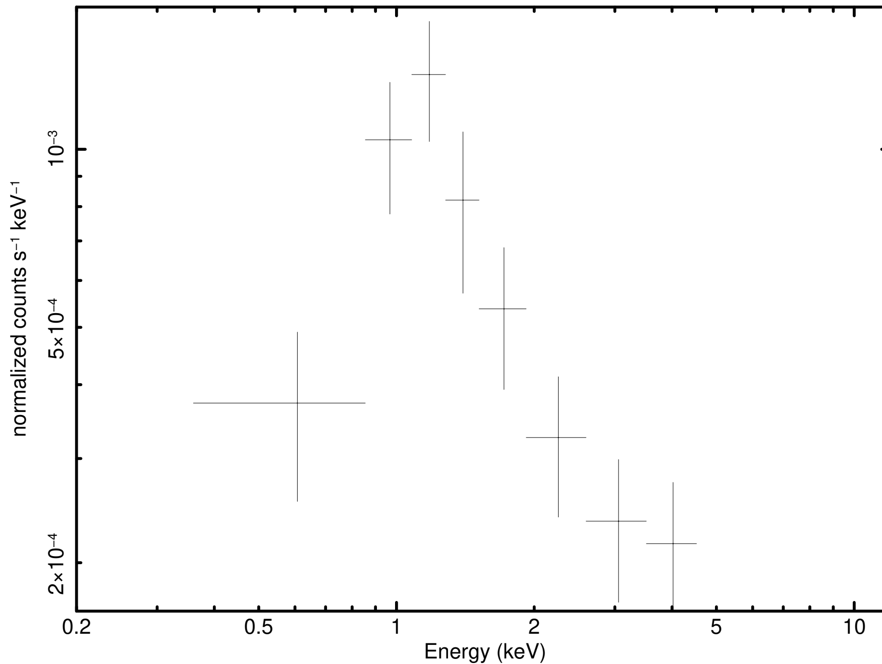
Source 42 minus background (P0931790101M2S002SRSPEC002A)
