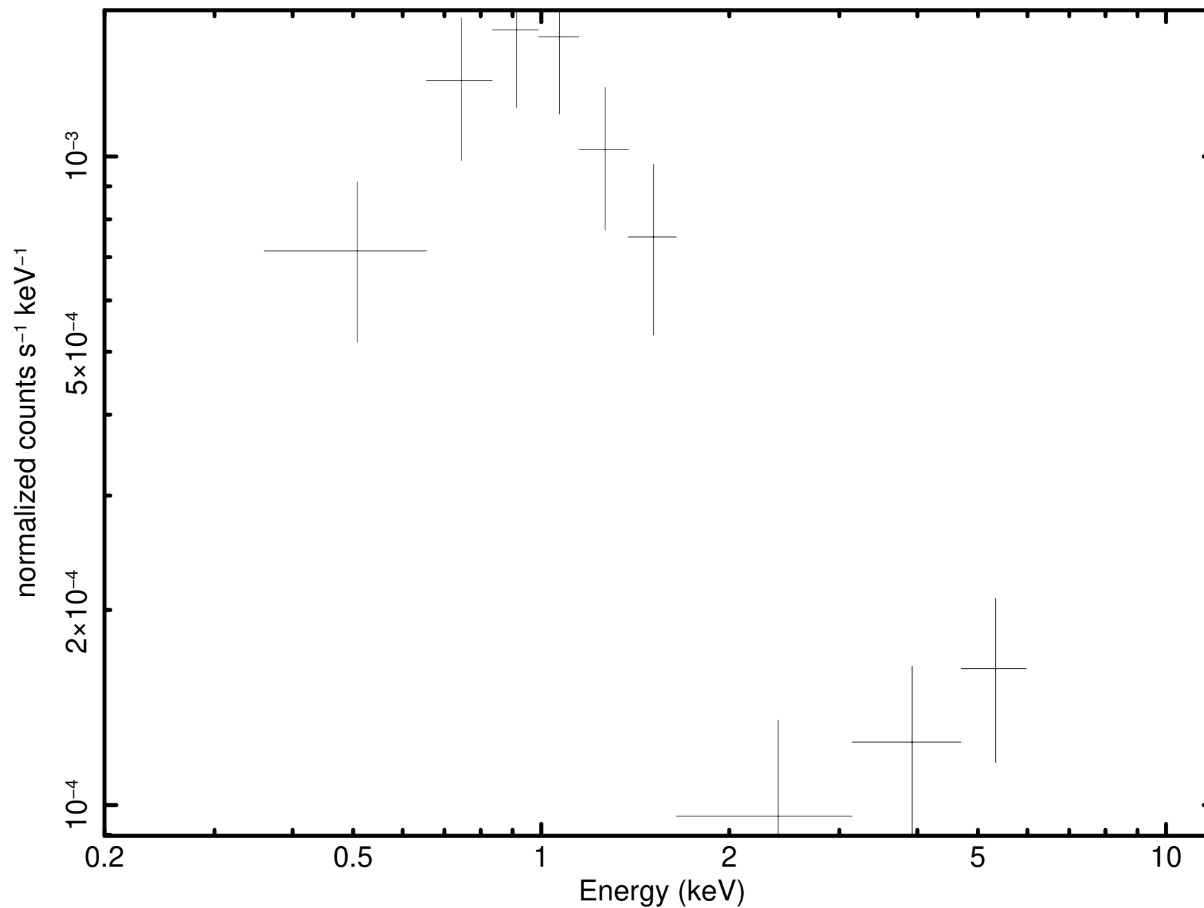
Source 109 minus background (P0931790101M2S002SRSPEC006D)
