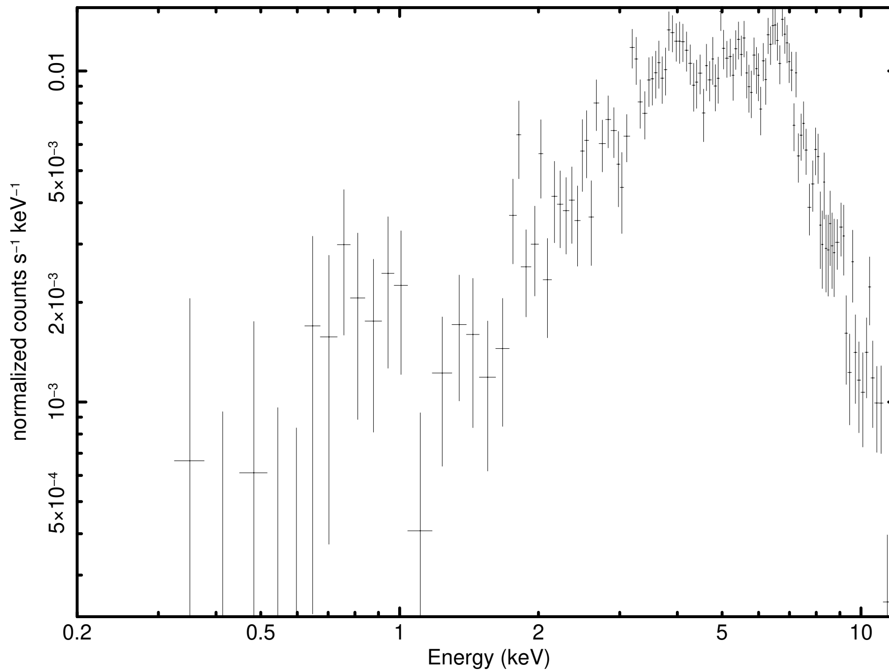
Source 1 minus background (P0931790101PNS003SRSPEC0001)
