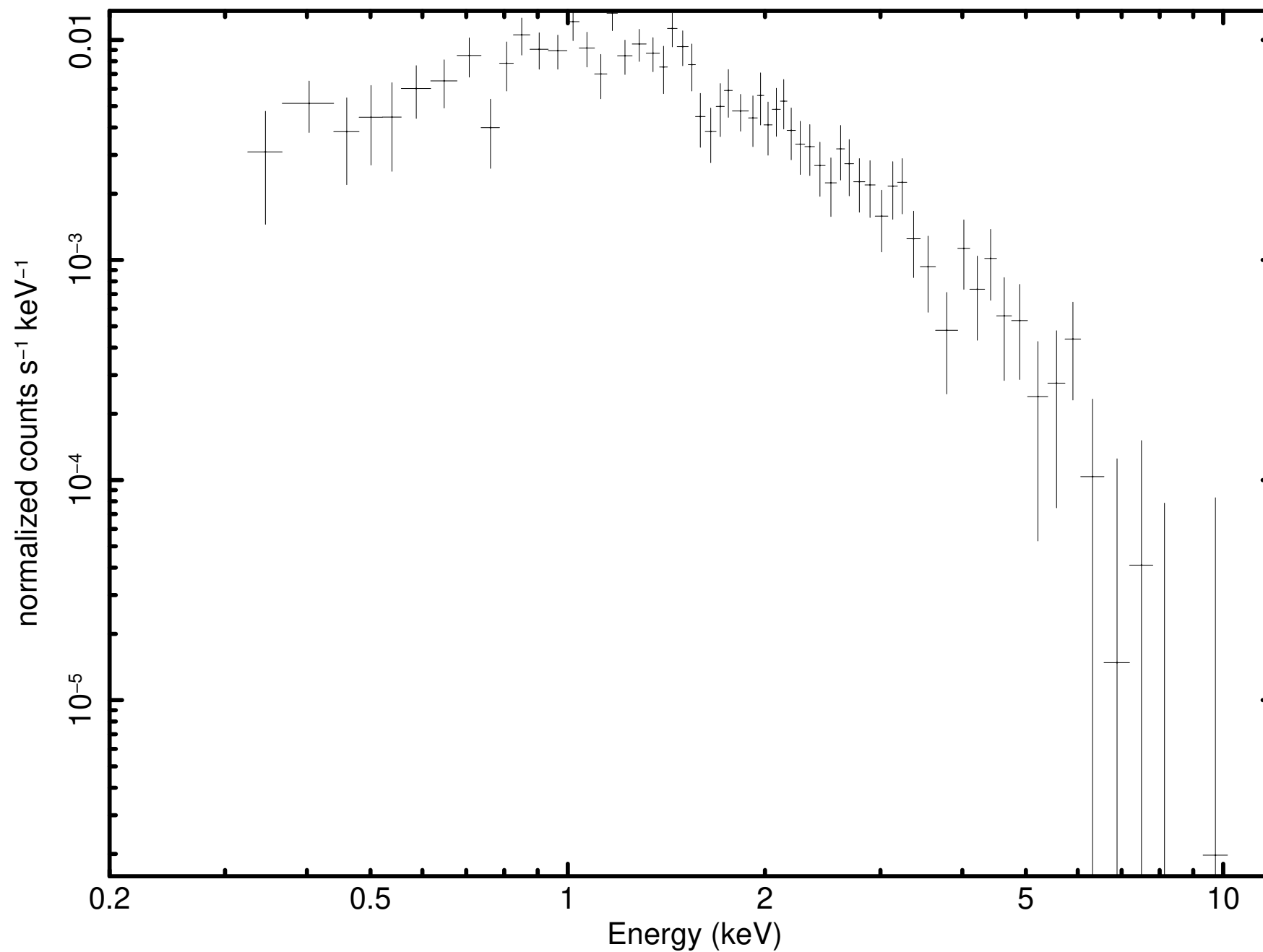
Source 6 minus background (P0931790101PNS003SRSPEC0006)
