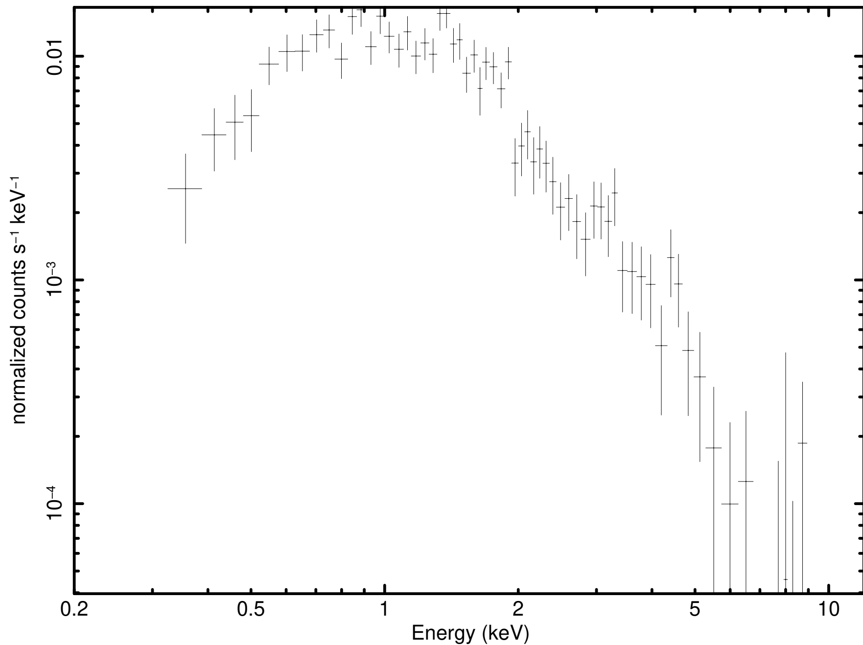
Source 9 minus background (P0931790101PNS003SRSPEC0009)
