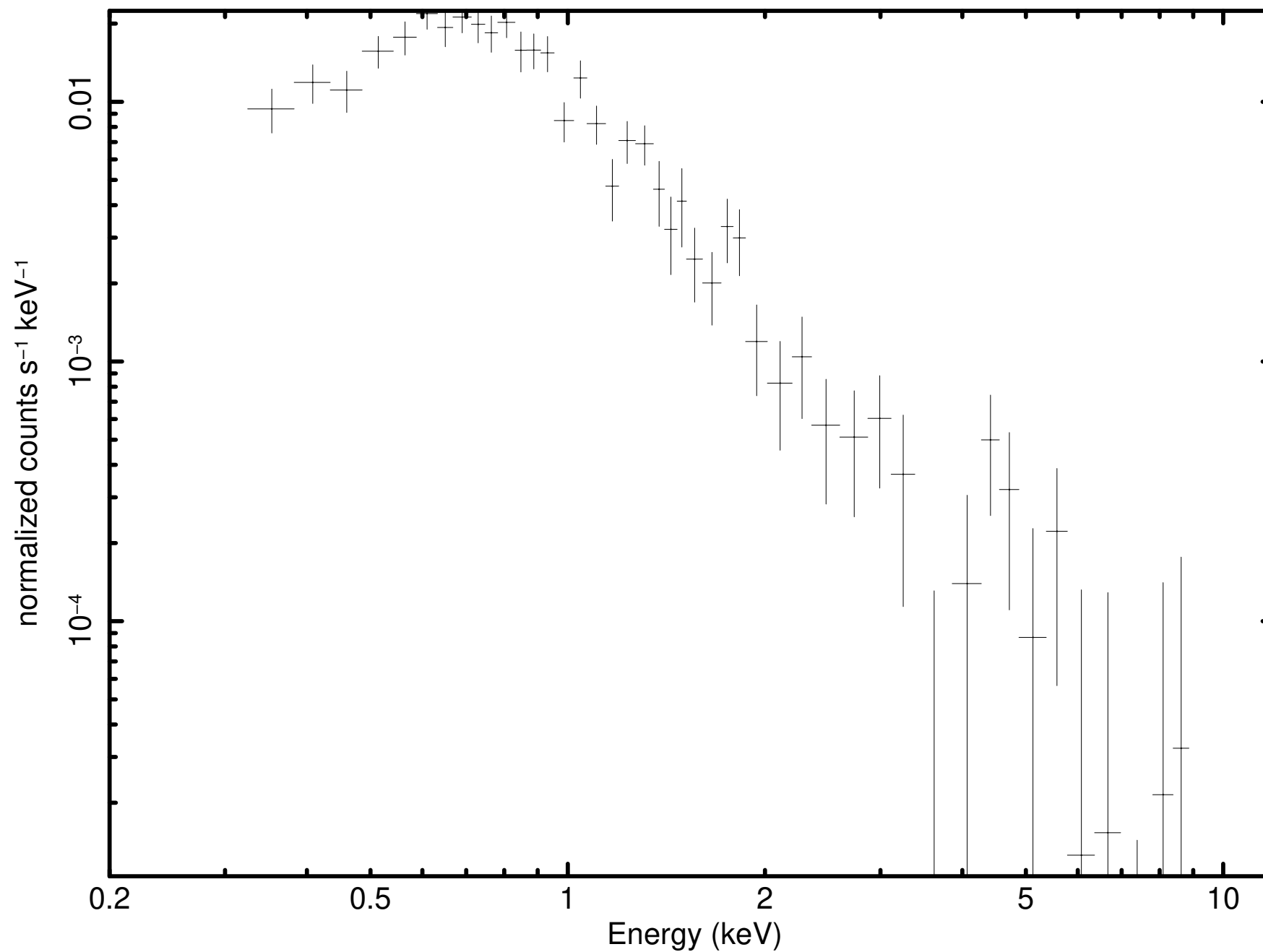
Source 11 minus background (P0931790101PNS003SRSPEC000B)
