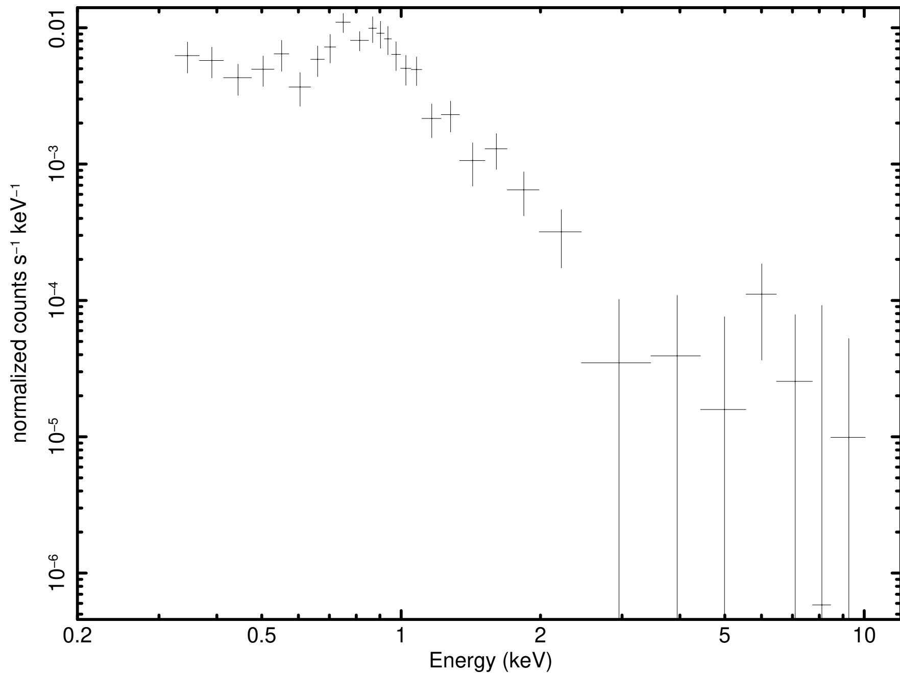
Source 14 minus background (P0931790101PNS003SRSPEC000E)
