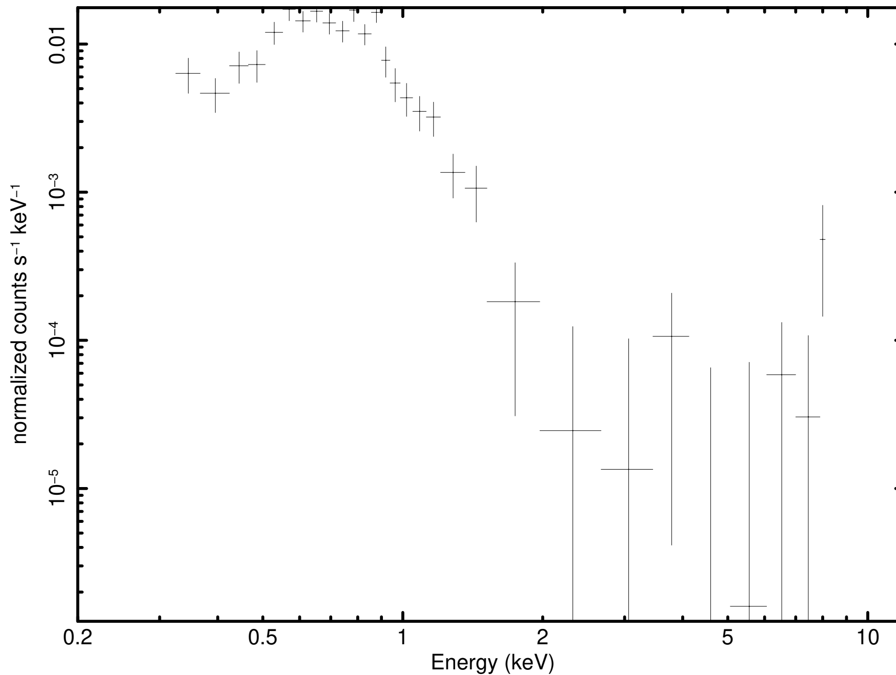
Source 15 minus background (P0931790101PNS003SRSPEC000F)
