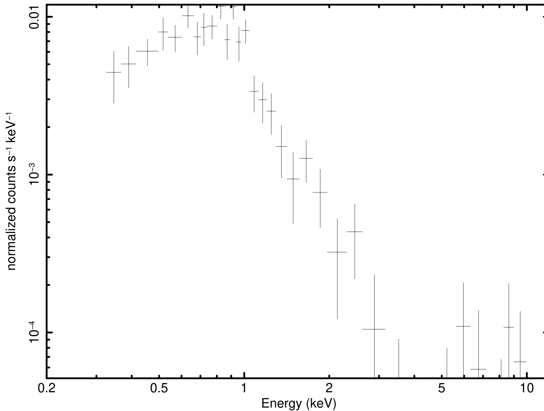
Source 16 minus background (P0931790101PNS003SRSPEC0010)
