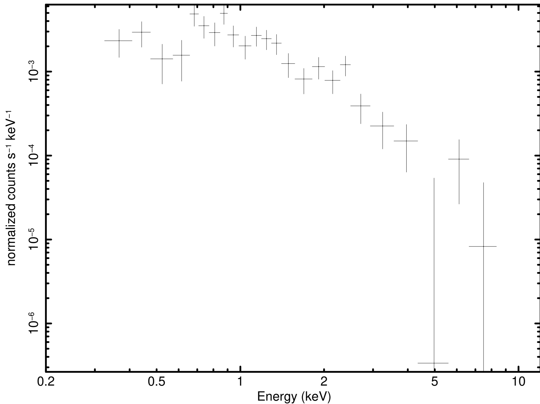
Source 17 minus background (P0931790101PNS003SRSPEC0011)
