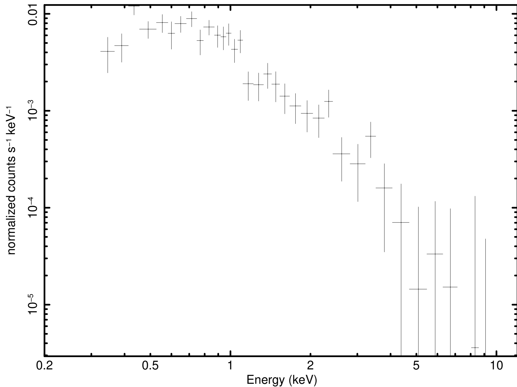
Source 18 minus background (P0931790101PNS003SRSPEC0012)
