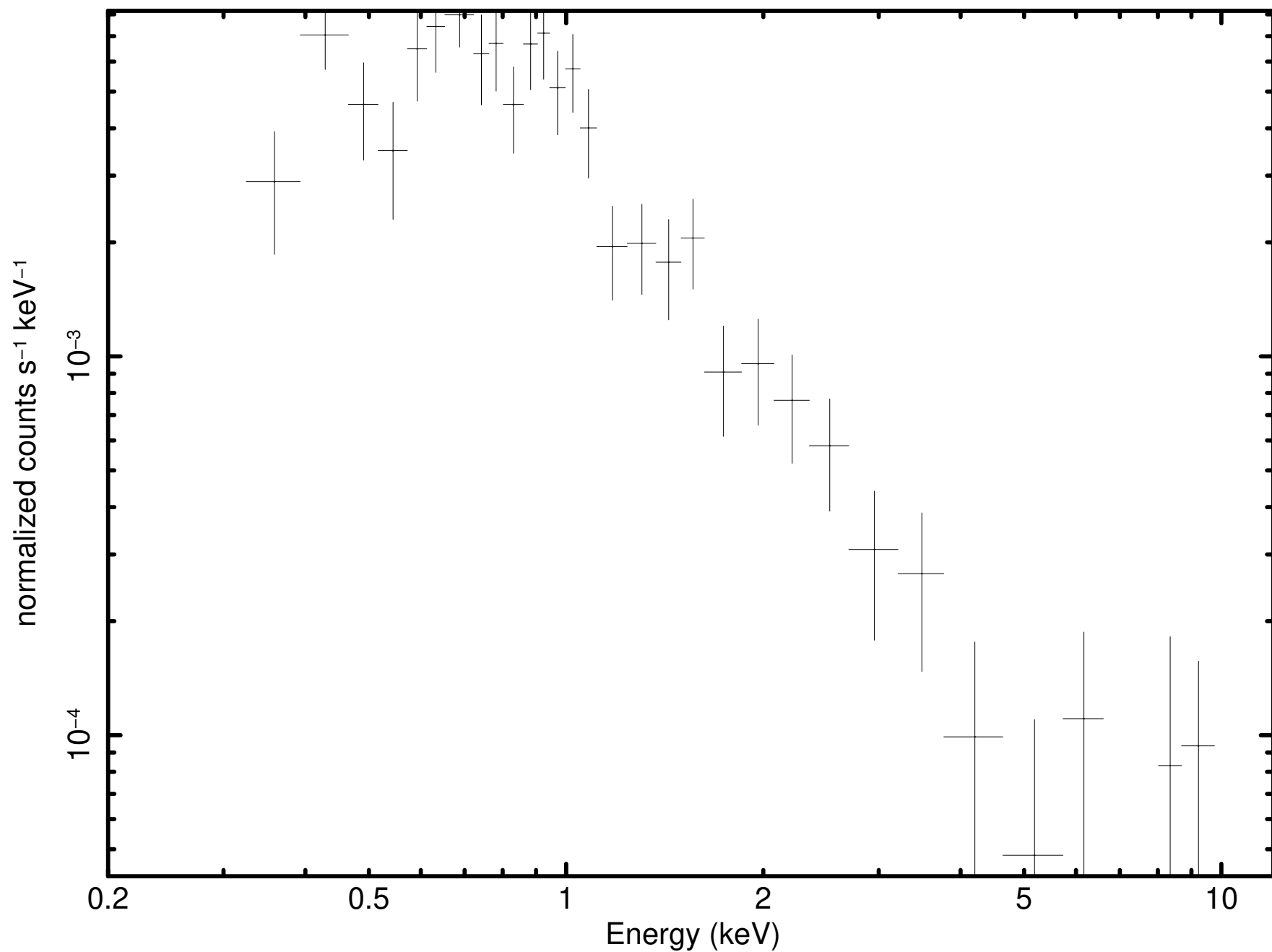
Source 19 minus background (P0931790101PNS003SRSPEC0013)
