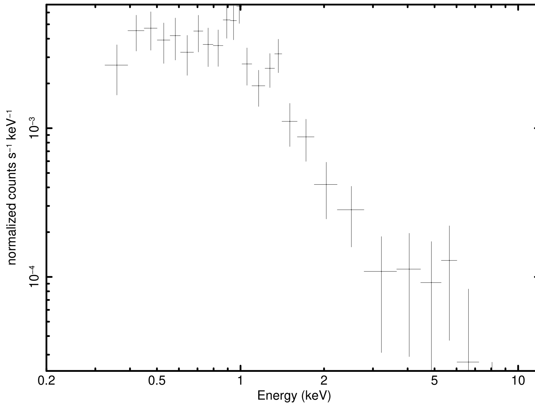
Source 20 minus background (P0931790101PNS003SRSPEC0014)
