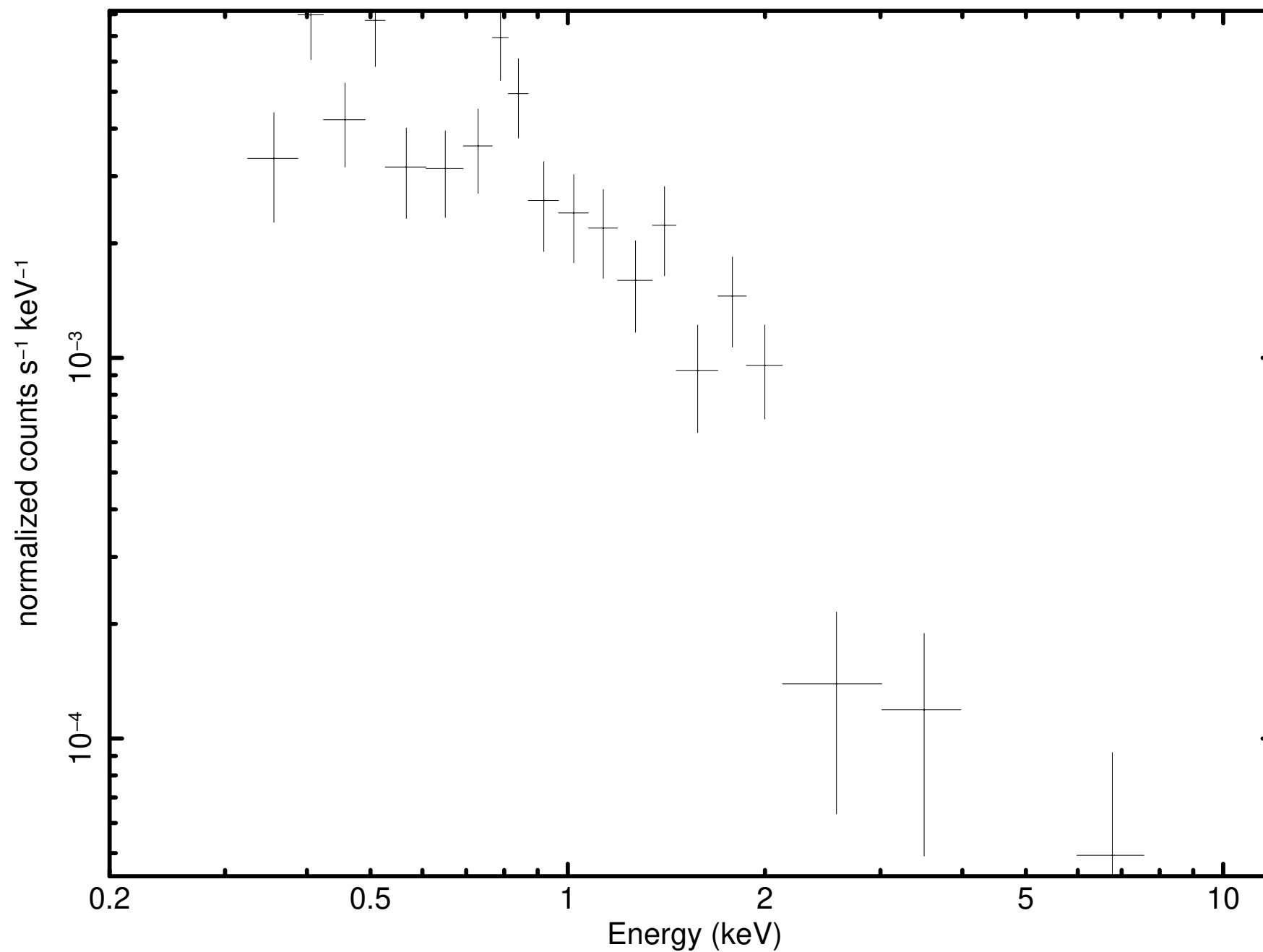
Source 21 minus background (P0931790101PNS003SRSPEC0015)
