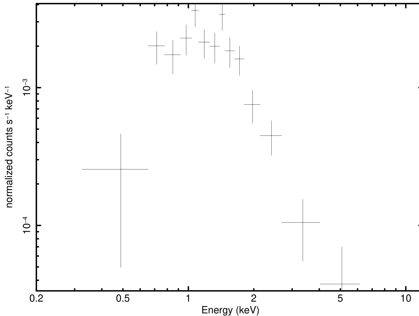
Source 22 minus background (P0931790101PNS003SRSPEC0016)
