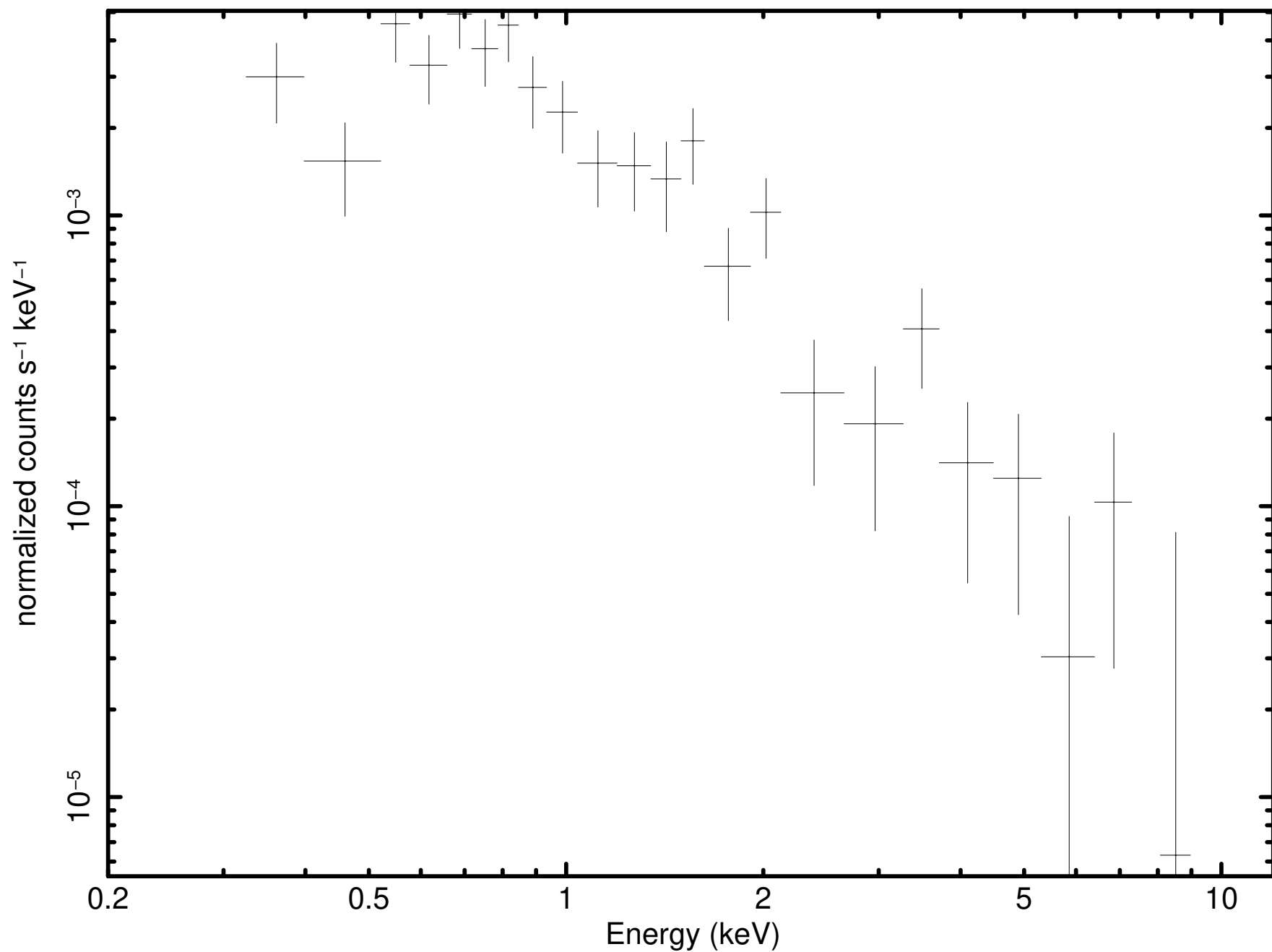
Source 23 minus background (P0931790101PNS003SRSPEC0017)
