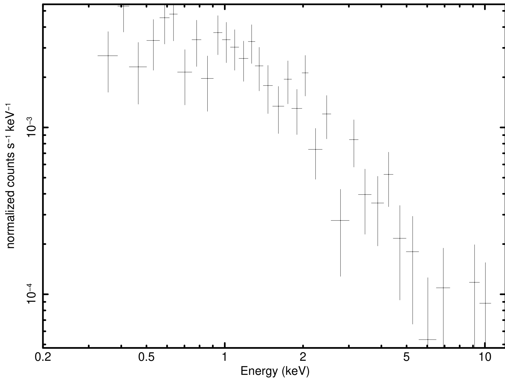
Source 24 minus background (P0931790101PNS003SRSPEC0018)
