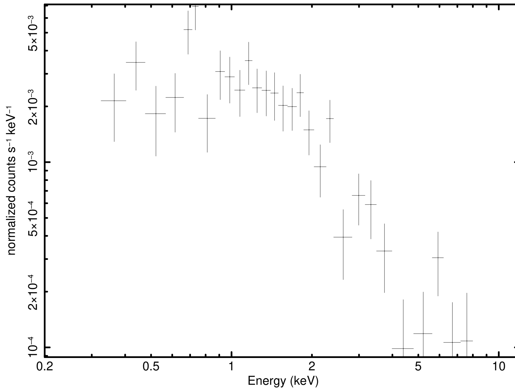
Source 26 minus background (P0931790101PNS003SRSPEC001A)
