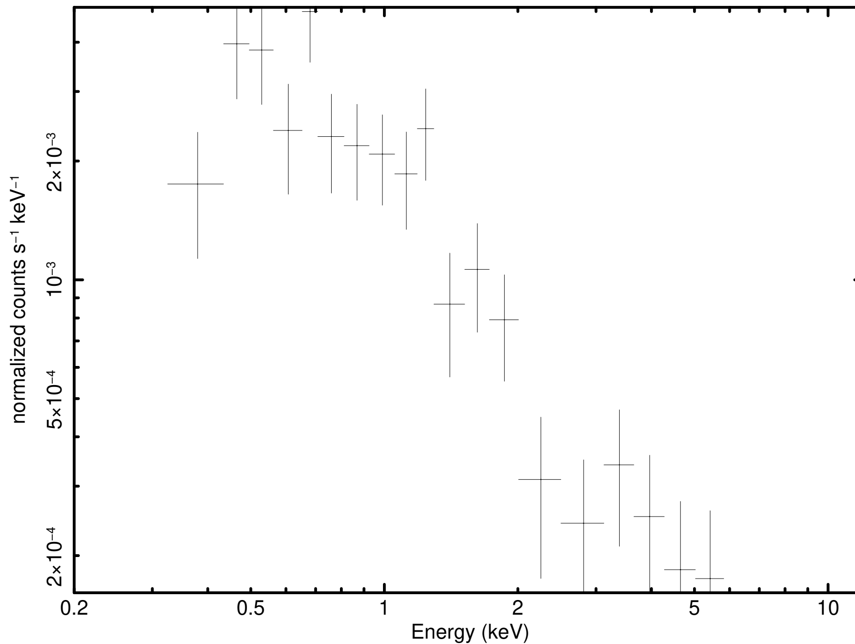
Source 30 minus background (P0931790101PNS003SRSPEC001E)
