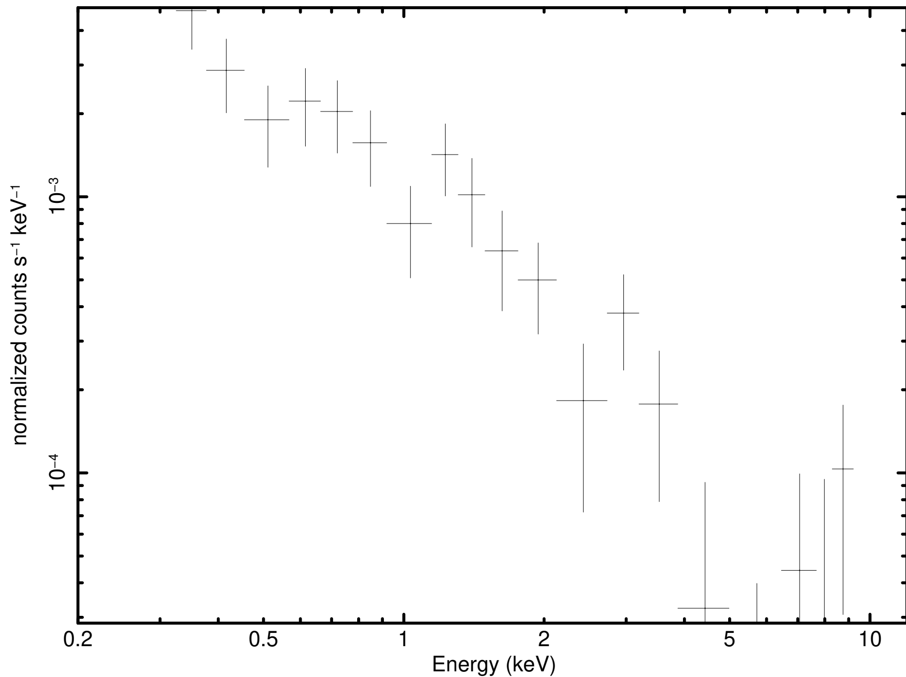
Source 31 minus background (P0931790101PNS003SRSPEC001F)
