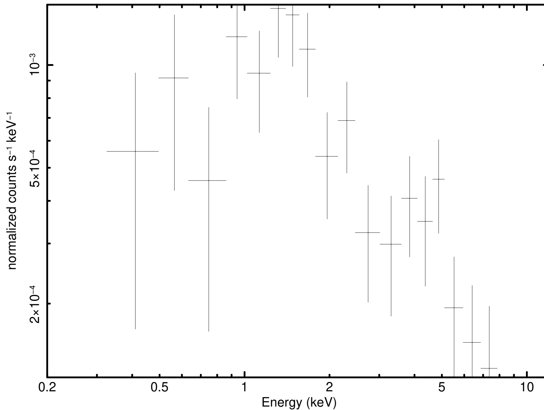
Source 32 minus background (P0931790101PNS003SRSPEC0020)
