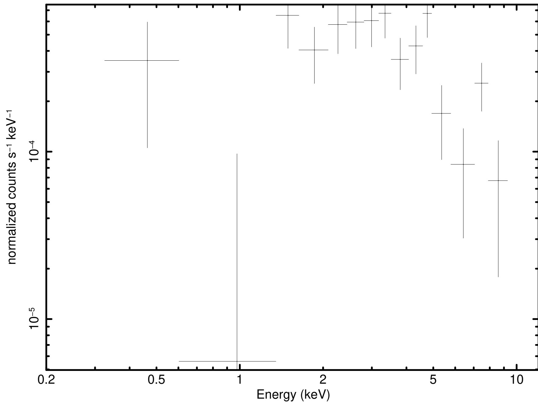
Source 33 minus background (P0931790101PNS003SRSPEC0021)
