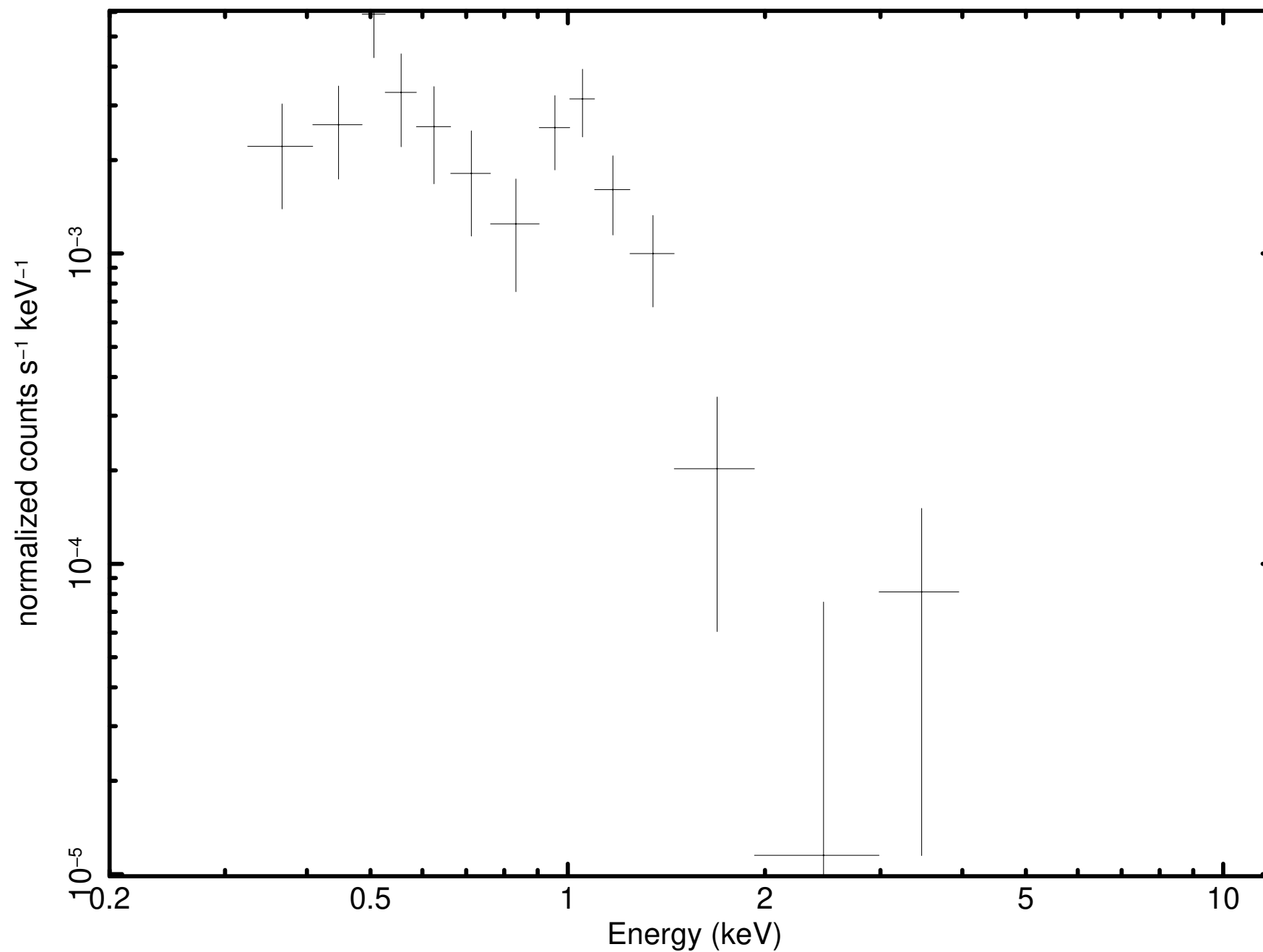
Source 35 minus background (P0931790101PNS003SRSPEC0023)
