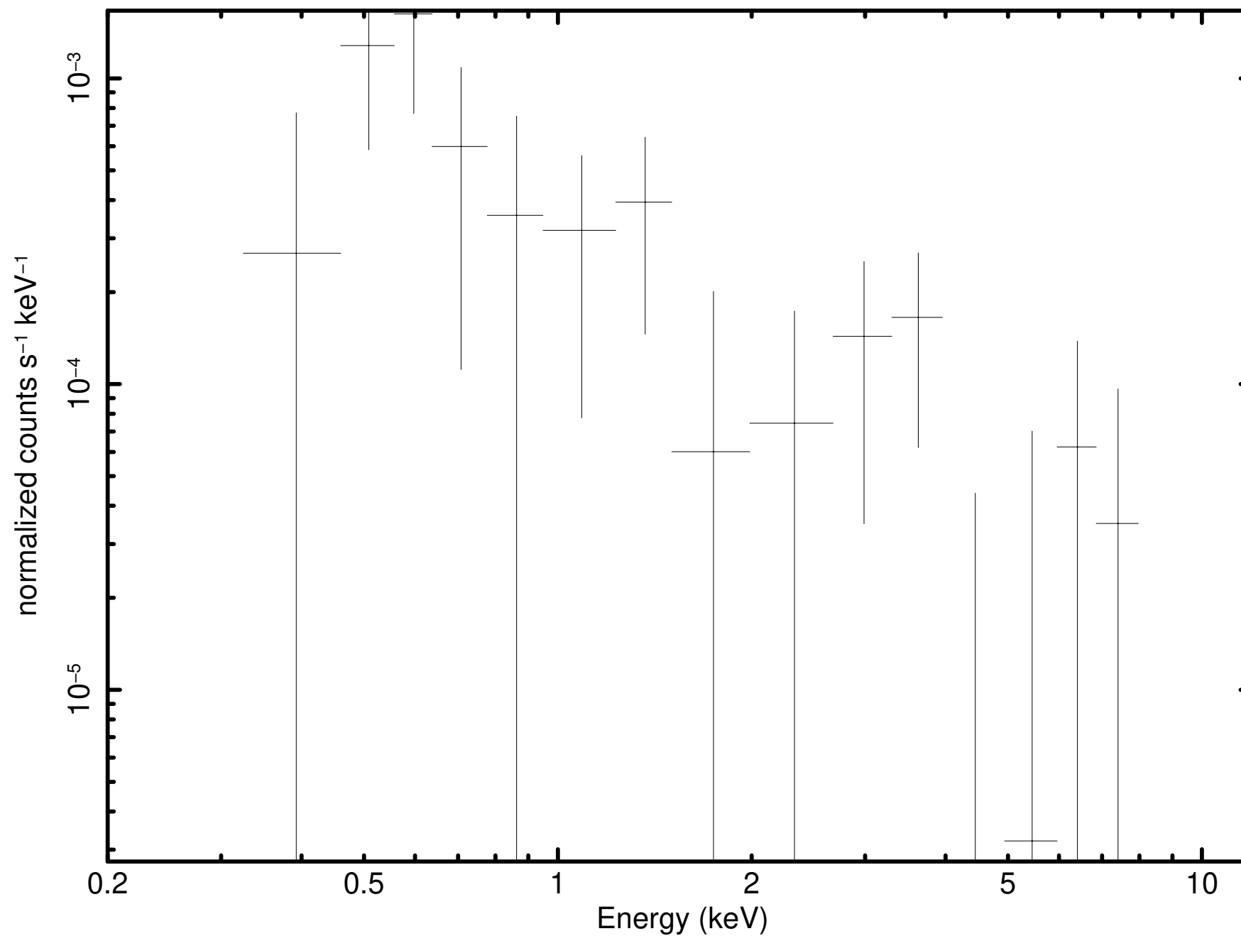
Source 36 minus background (P0931790101PNS003SRSPEC0024)
