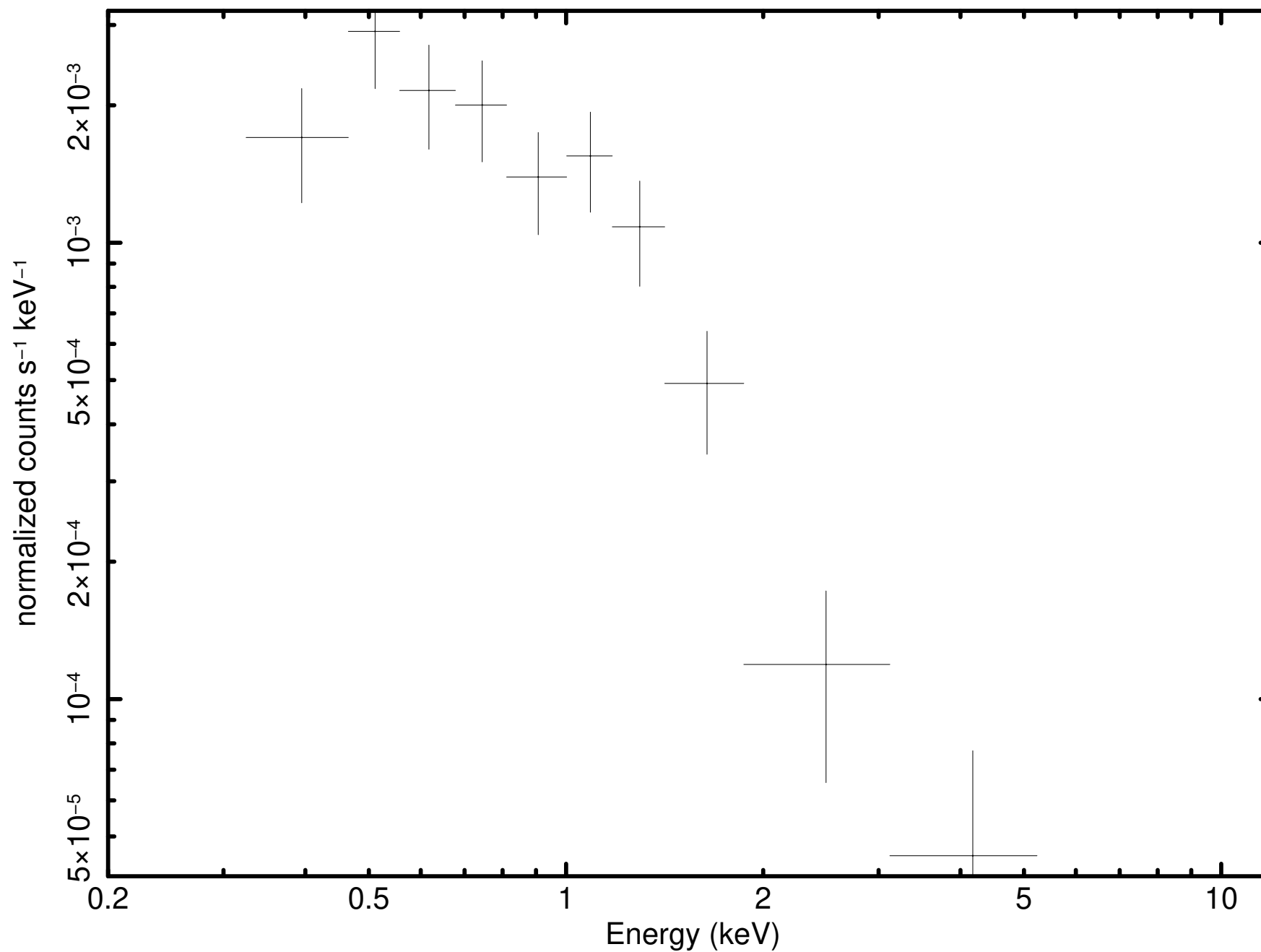
Source 37 minus background (P0931790101PNS003SRSPEC0025)
