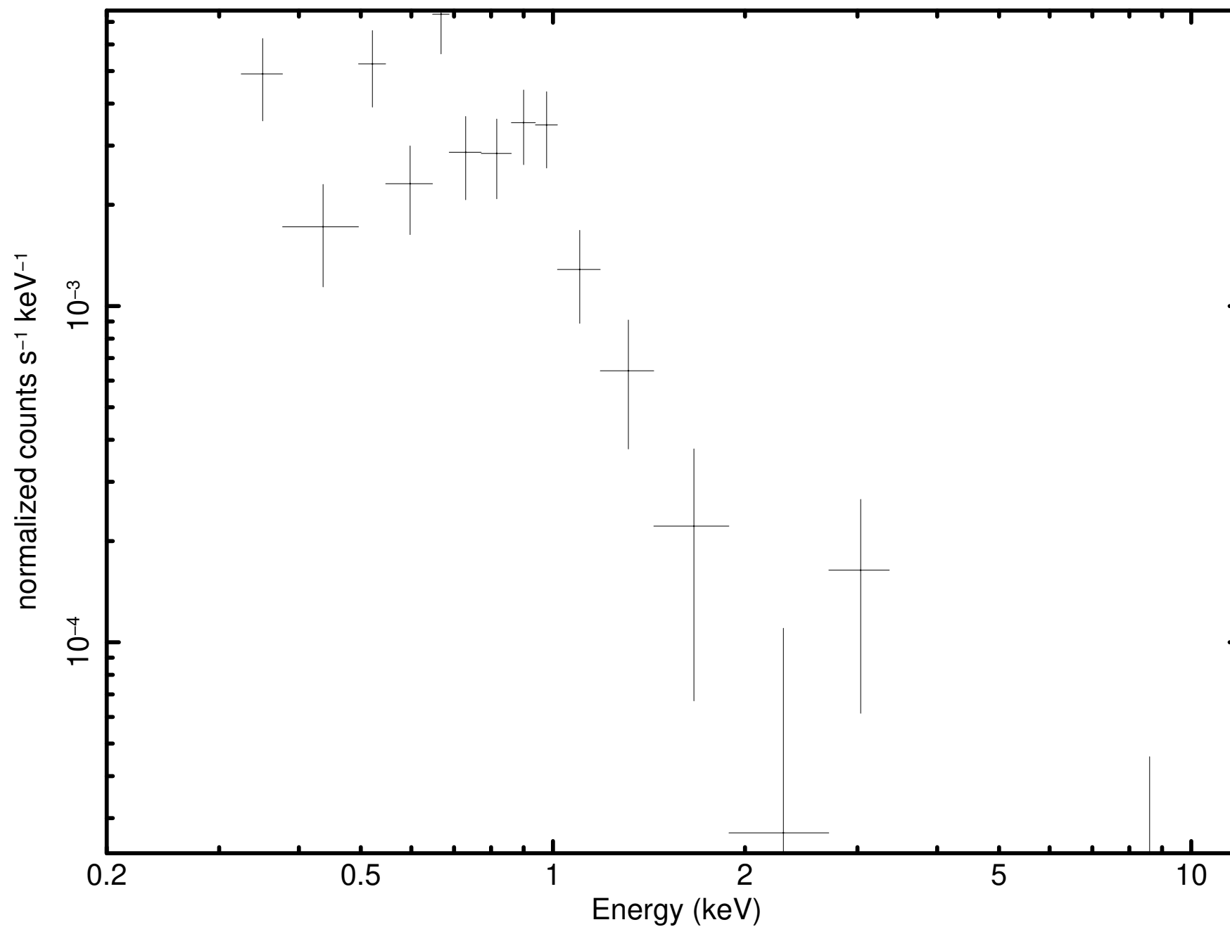
Source 38 minus background (P0931790101PNS003SRSPEC0026)
