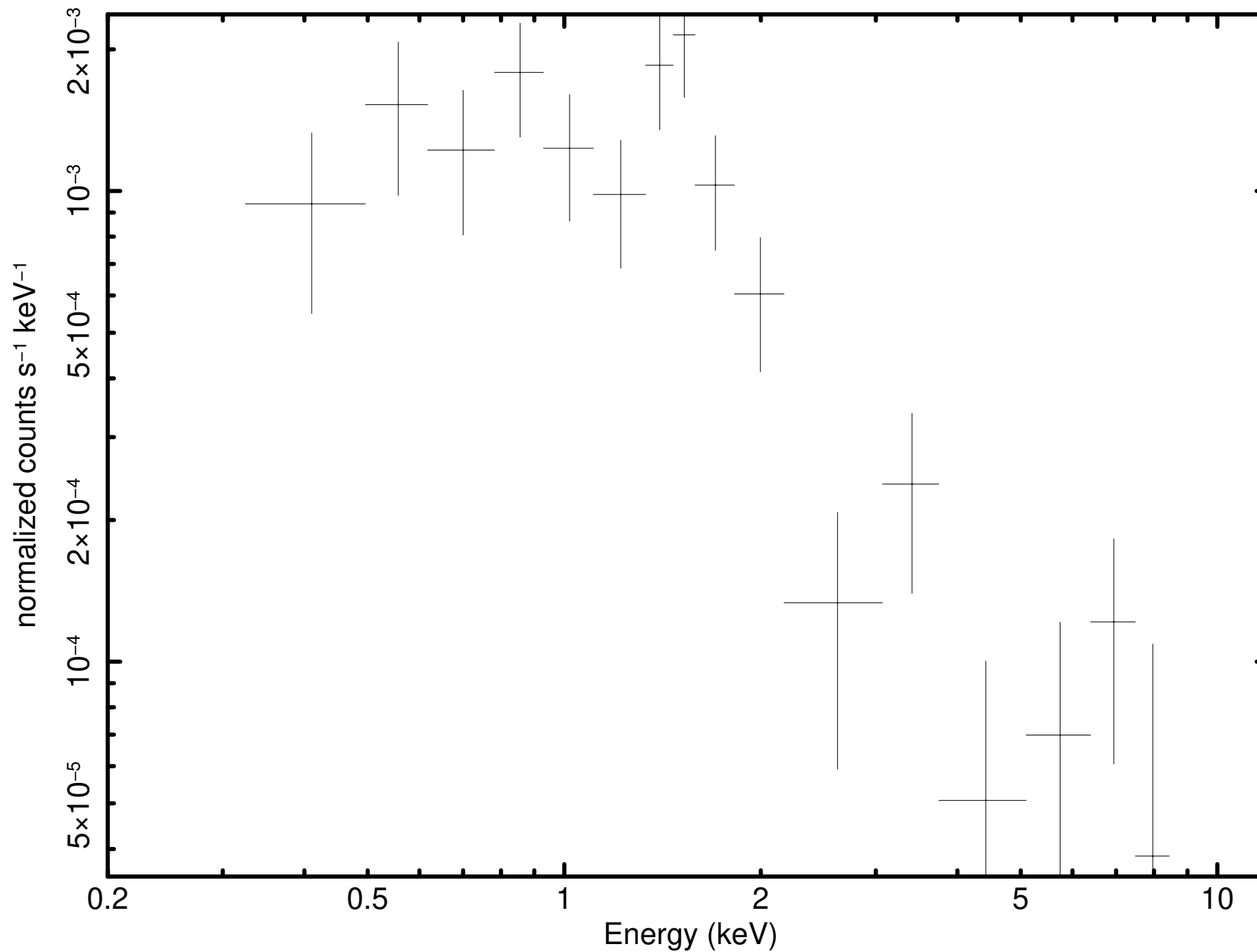
Source 39 minus background (P0931790101PNS003SRSPEC0027)
