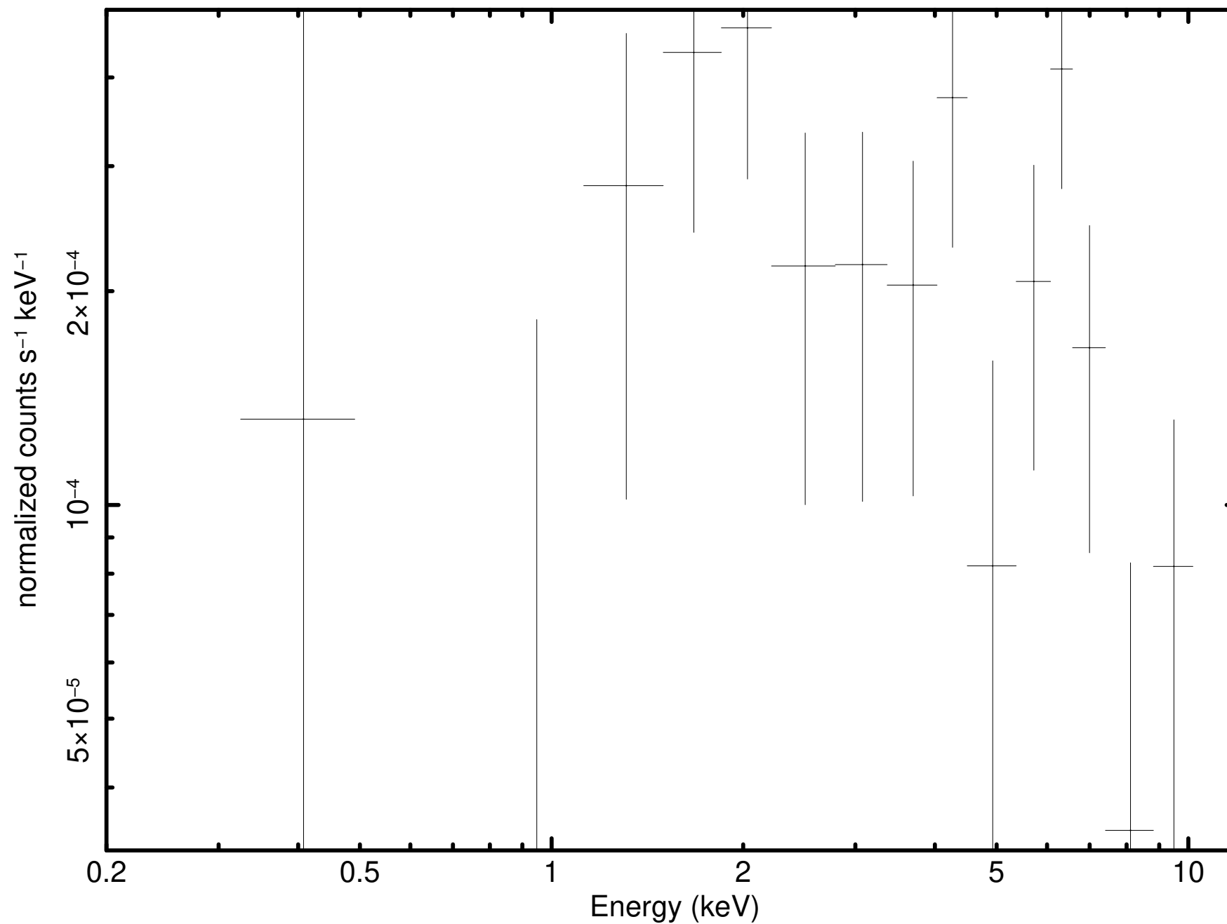
Source 40 minus background (P0931790101PNS003SRSPEC0028)
