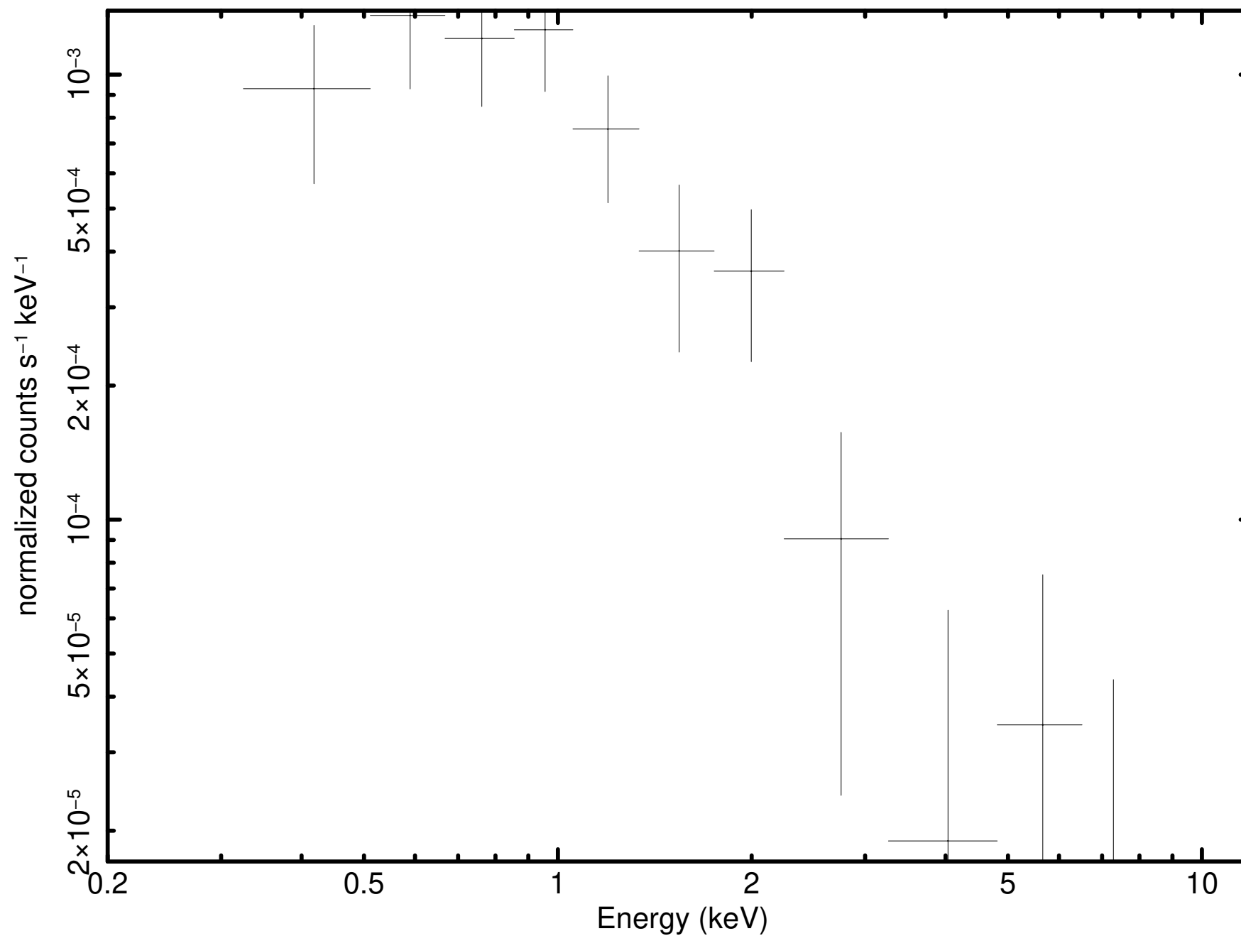
Source 43 minus background (P0931790101PNS003SRSPEC002B)
