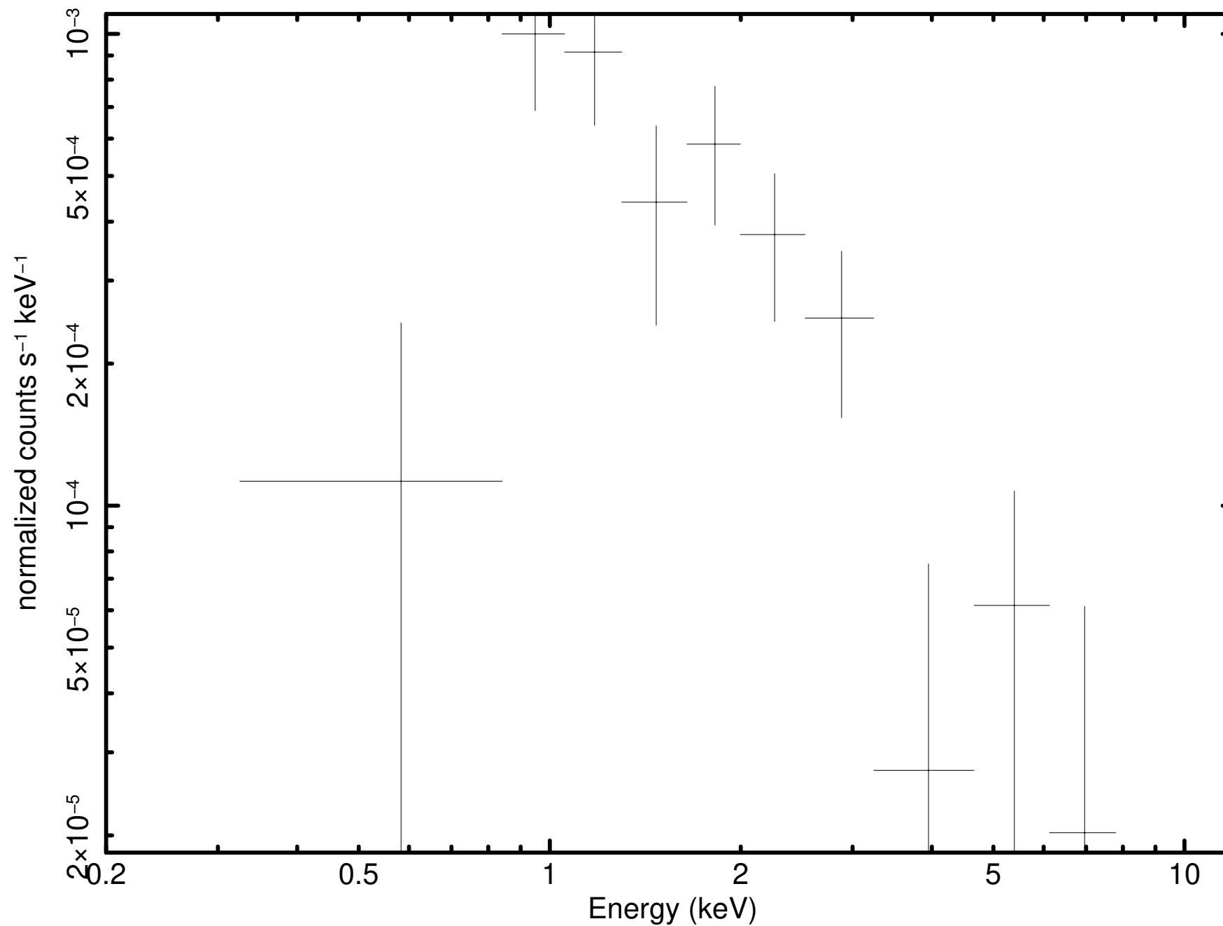
Source 44 minus background (P0931790101PNS003SRSPEC002C)
