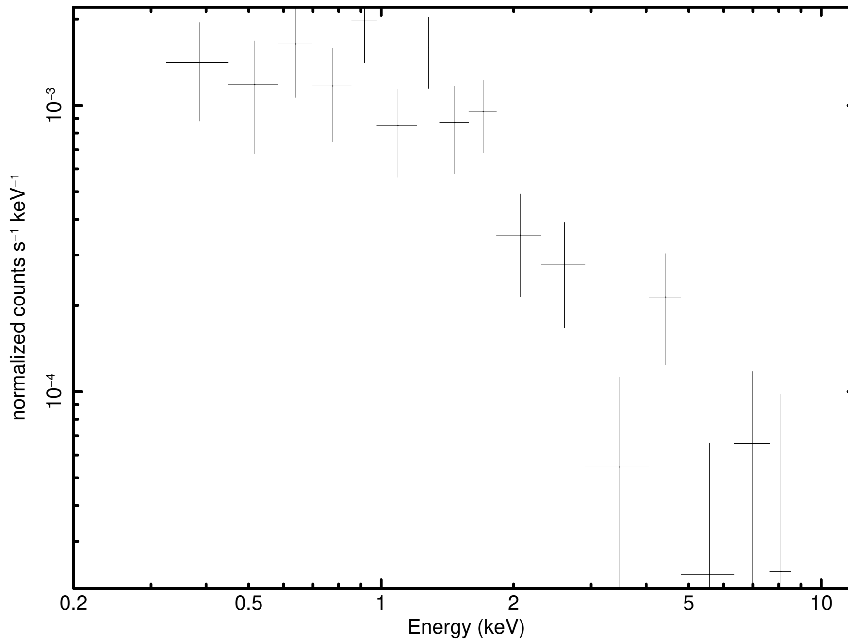
Source 45 minus background (P0931790101PNS003SRSPEC002D)
