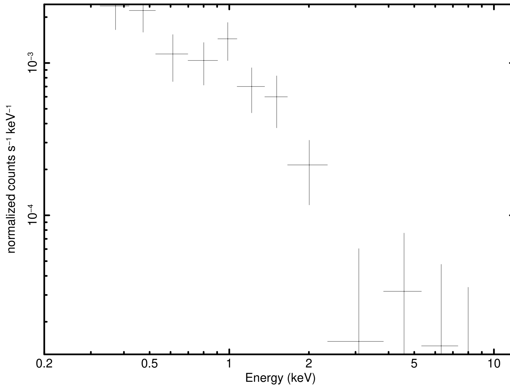
Source 46 minus background (P0931790101PNS003SRSPEC002E)
