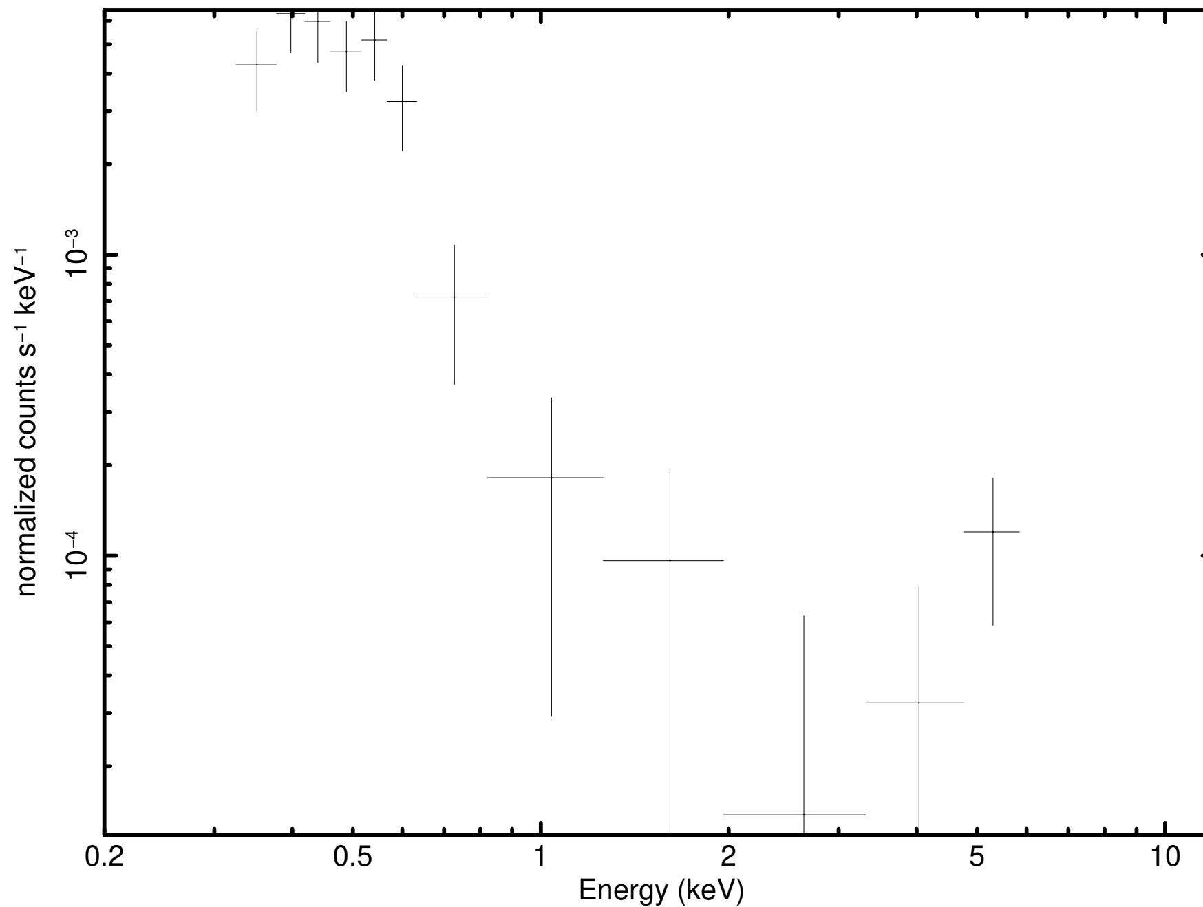
Source 47 minus background (P0931790101PNS003SRSPEC002F)
