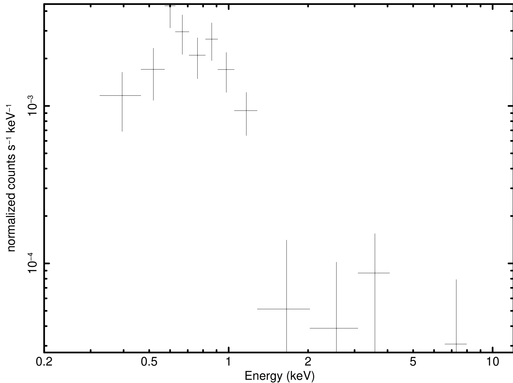
Source 48 minus background (P0931790101PNS003SRSPEC0030)
