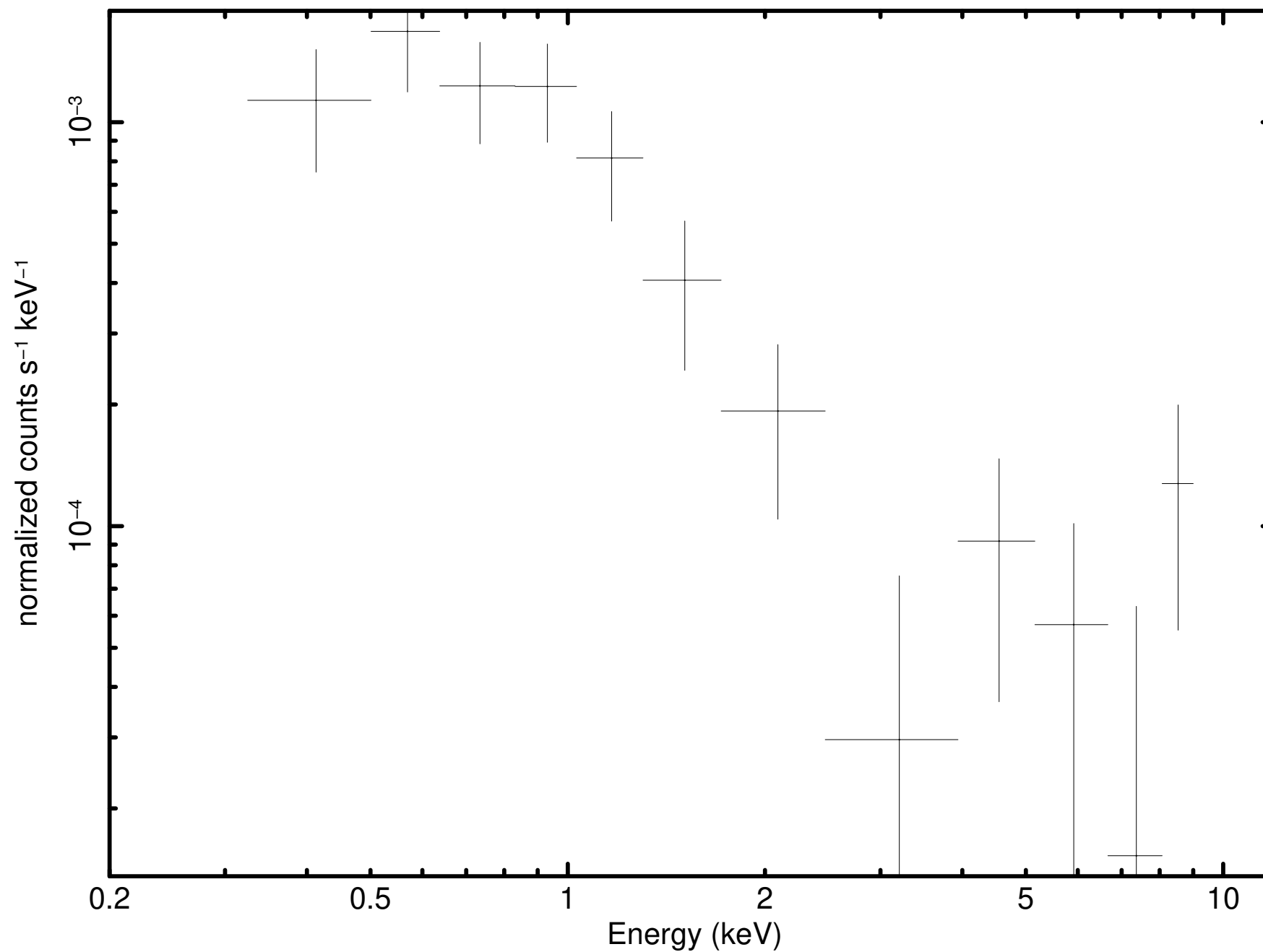
Source 51 minus background (P0931790101PNS003SRSPEC0033)
