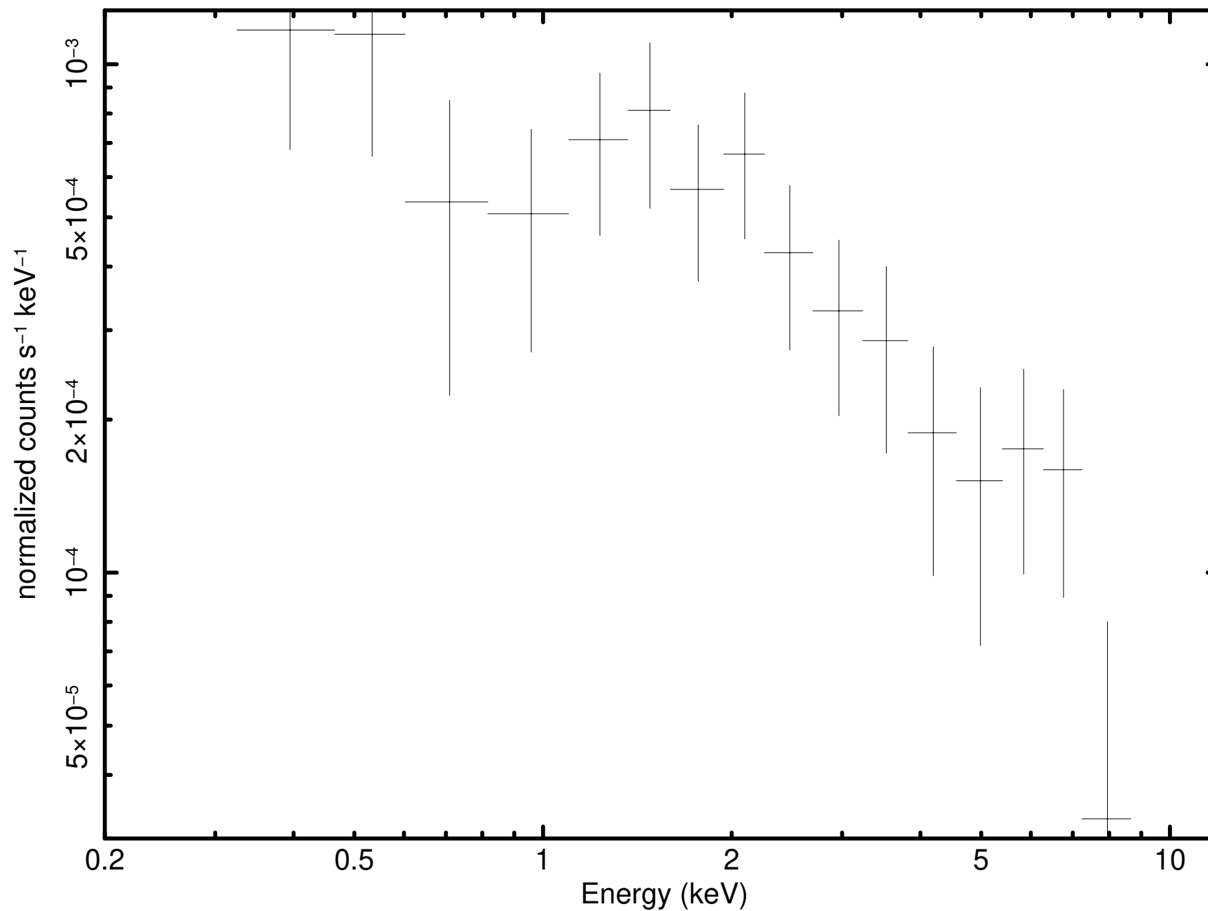
Source 53 minus background (P0931790101PNS003SRSPEC0035)
