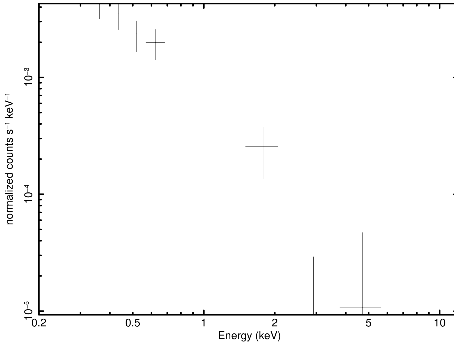
Source 56 minus background (P0931790101PNS003SRSPEC0038)
