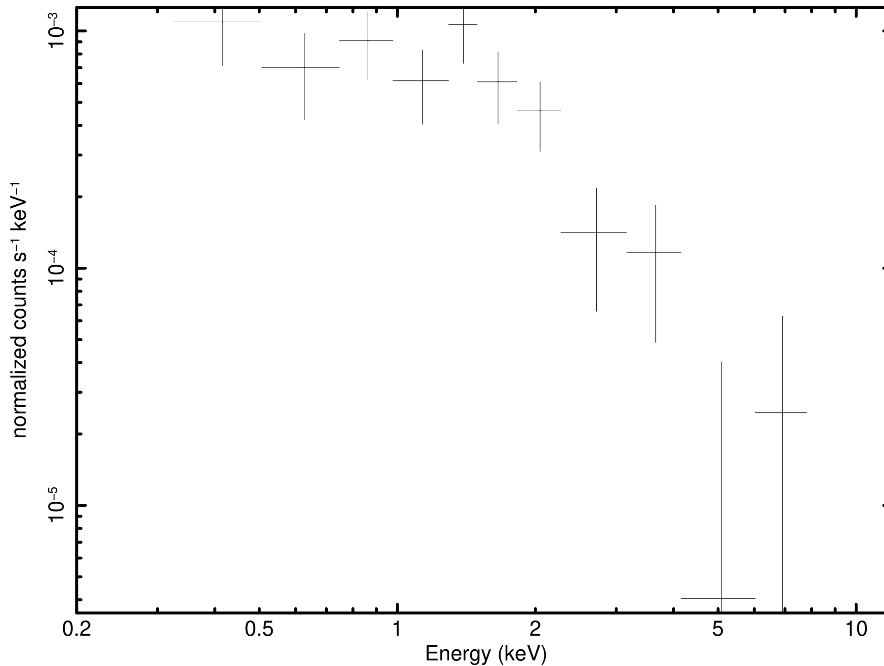
Source 57 minus background (P0931790101PNS003SRSPEC0039)
