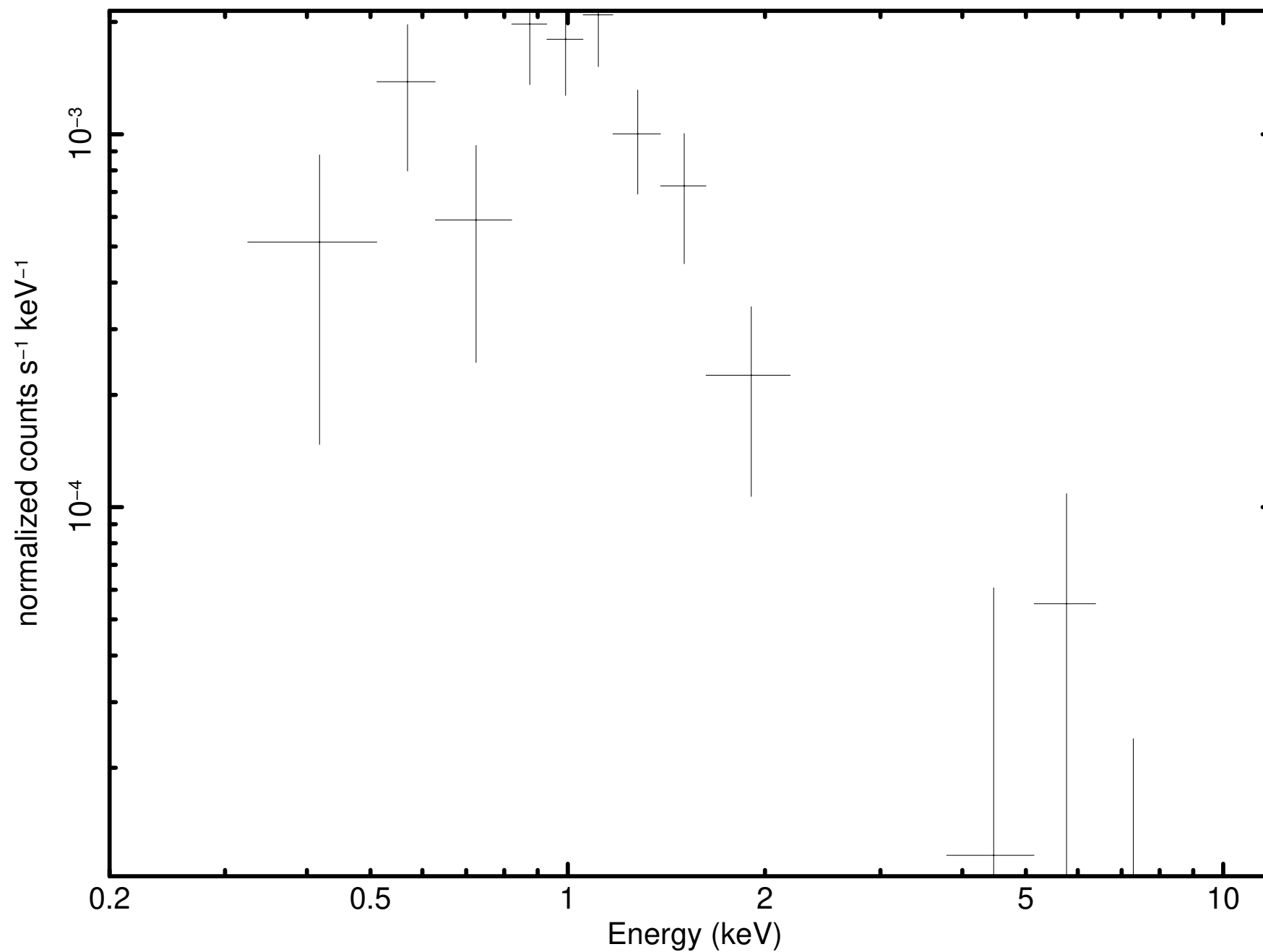
Source 60 minus background (P0931790101PNS003SRSPEC003C)
