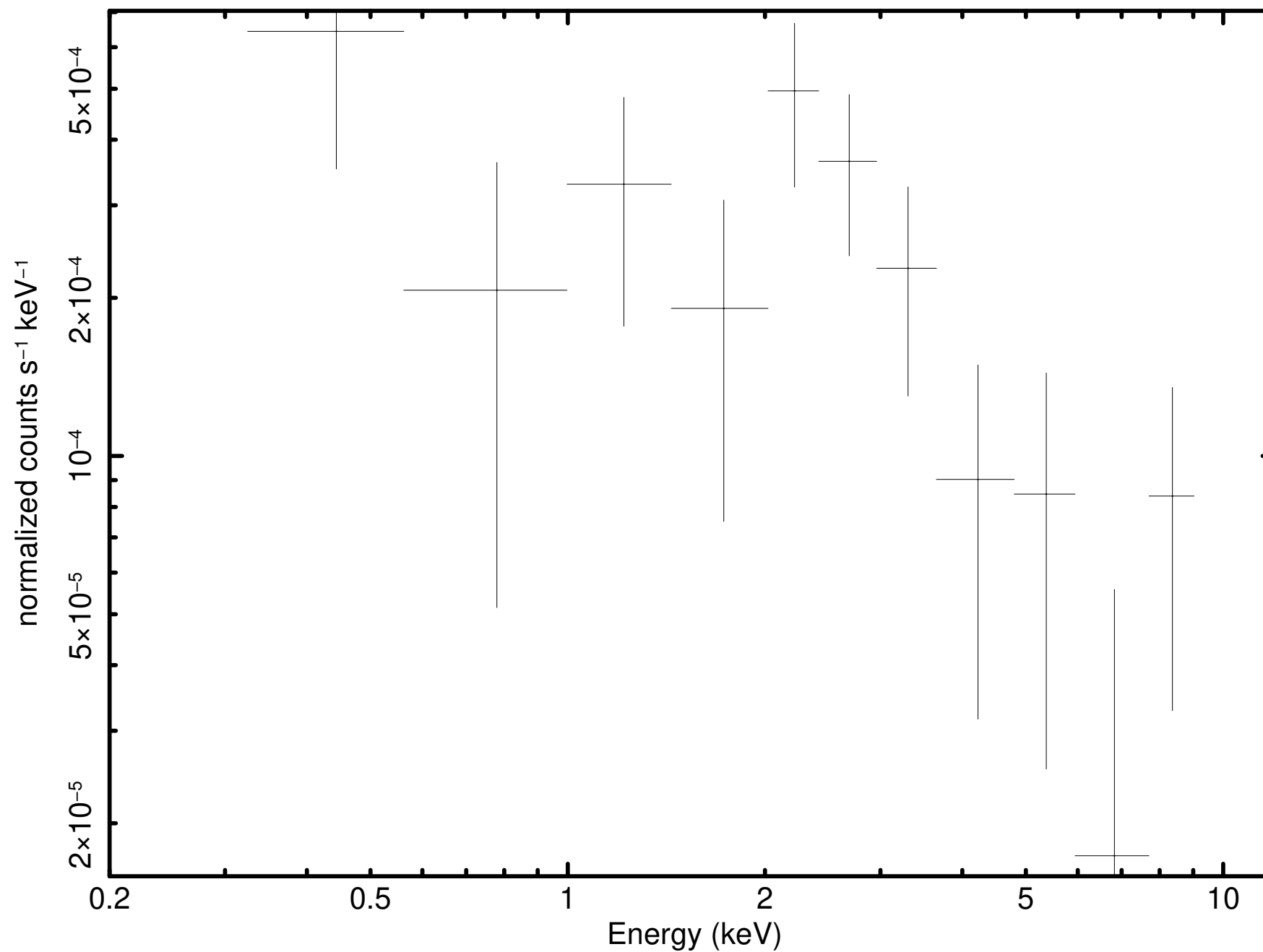
Source 61 minus background (P0931790101PNS003SRSPEC003D)
