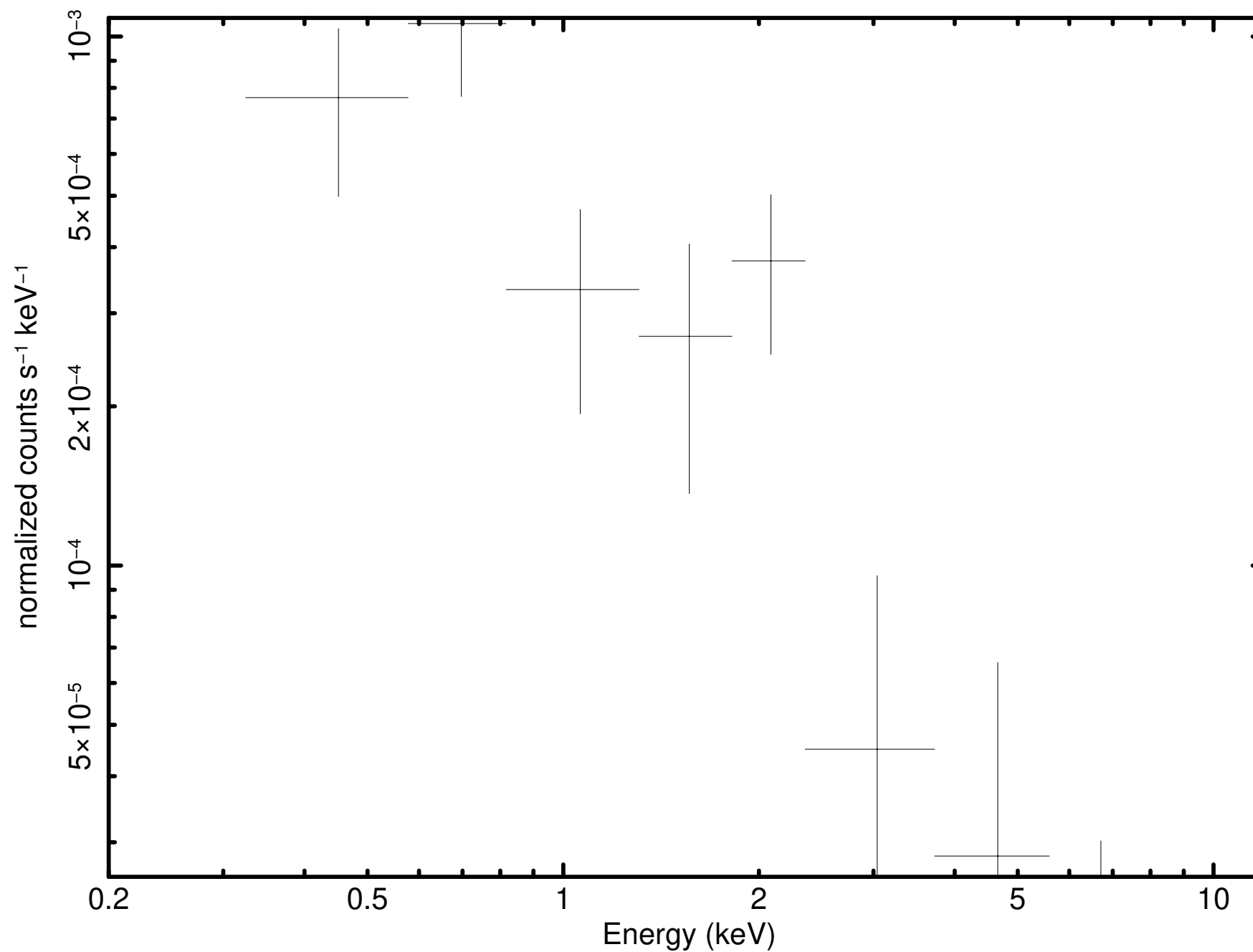
Source 63 minus background (P0931790101PNS003SRSPEC003F)
