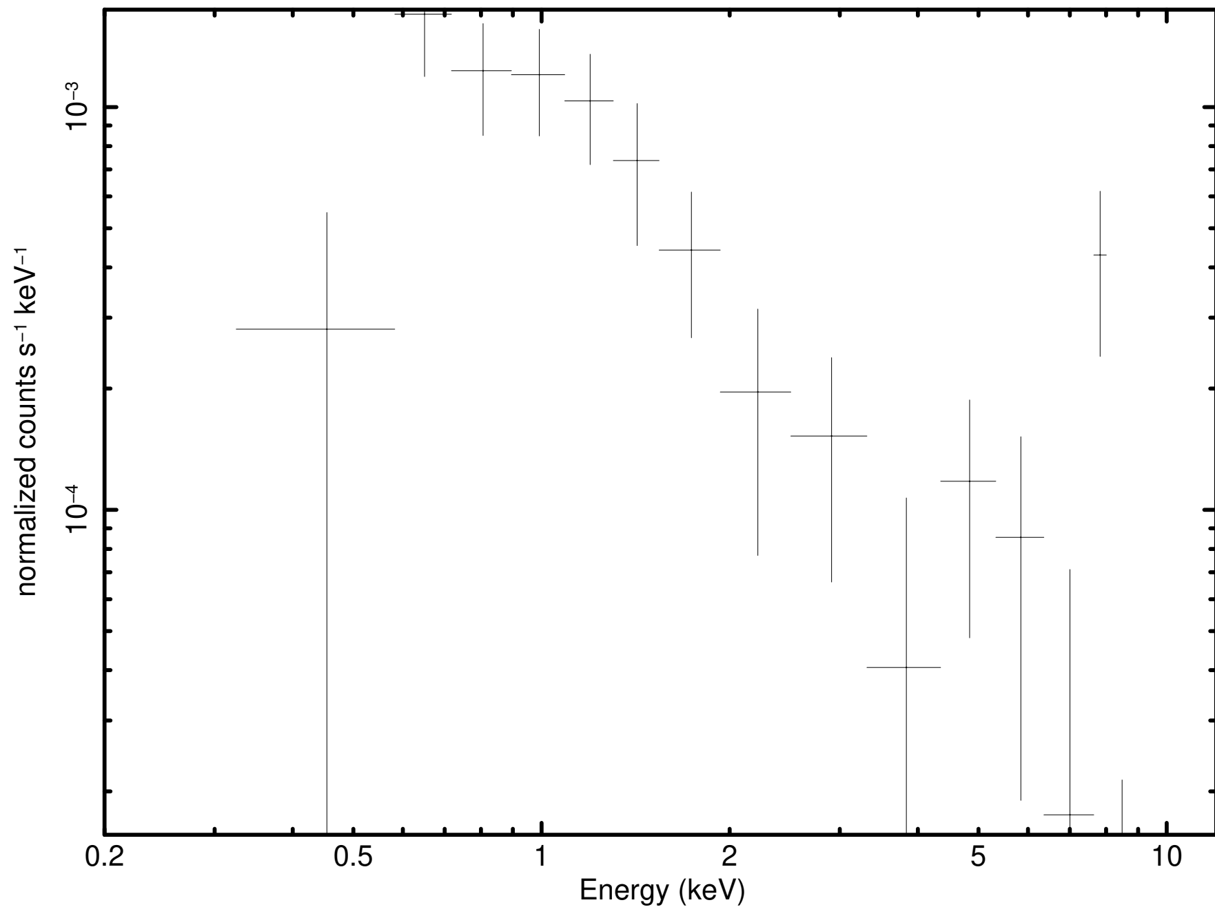
Source 65 minus background (P0931790101PNS003SRSPEC0041)
