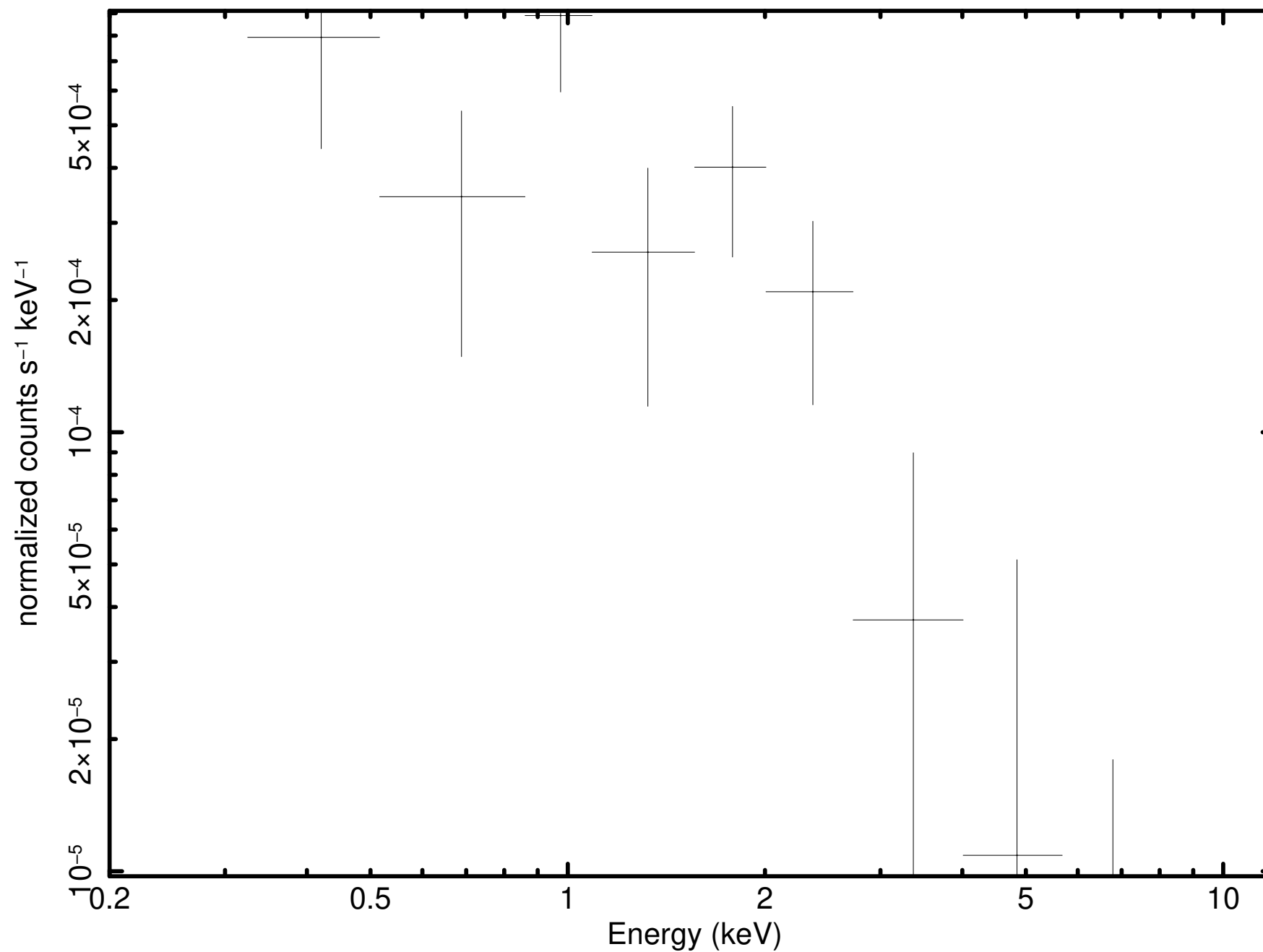
Source 66 minus background (P0931790101PNS003SRSPEC0042)
