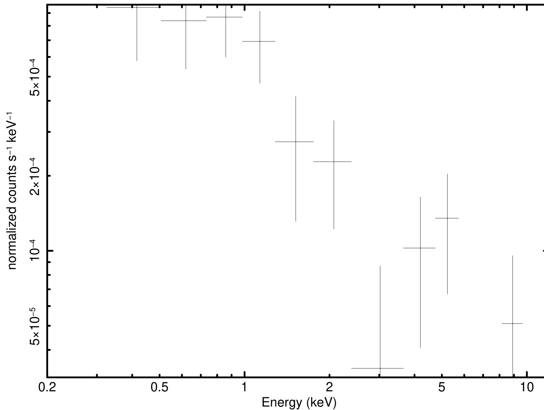
Source 68 minus background (P0931790101PNS003SRSPEC0044)
