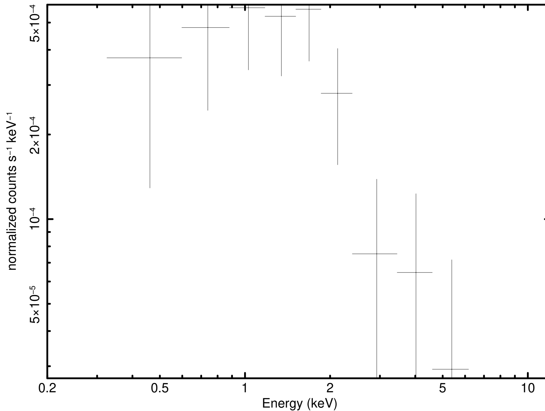
Source 74 minus background (P0931790101PNS003SRSPEC004A)
