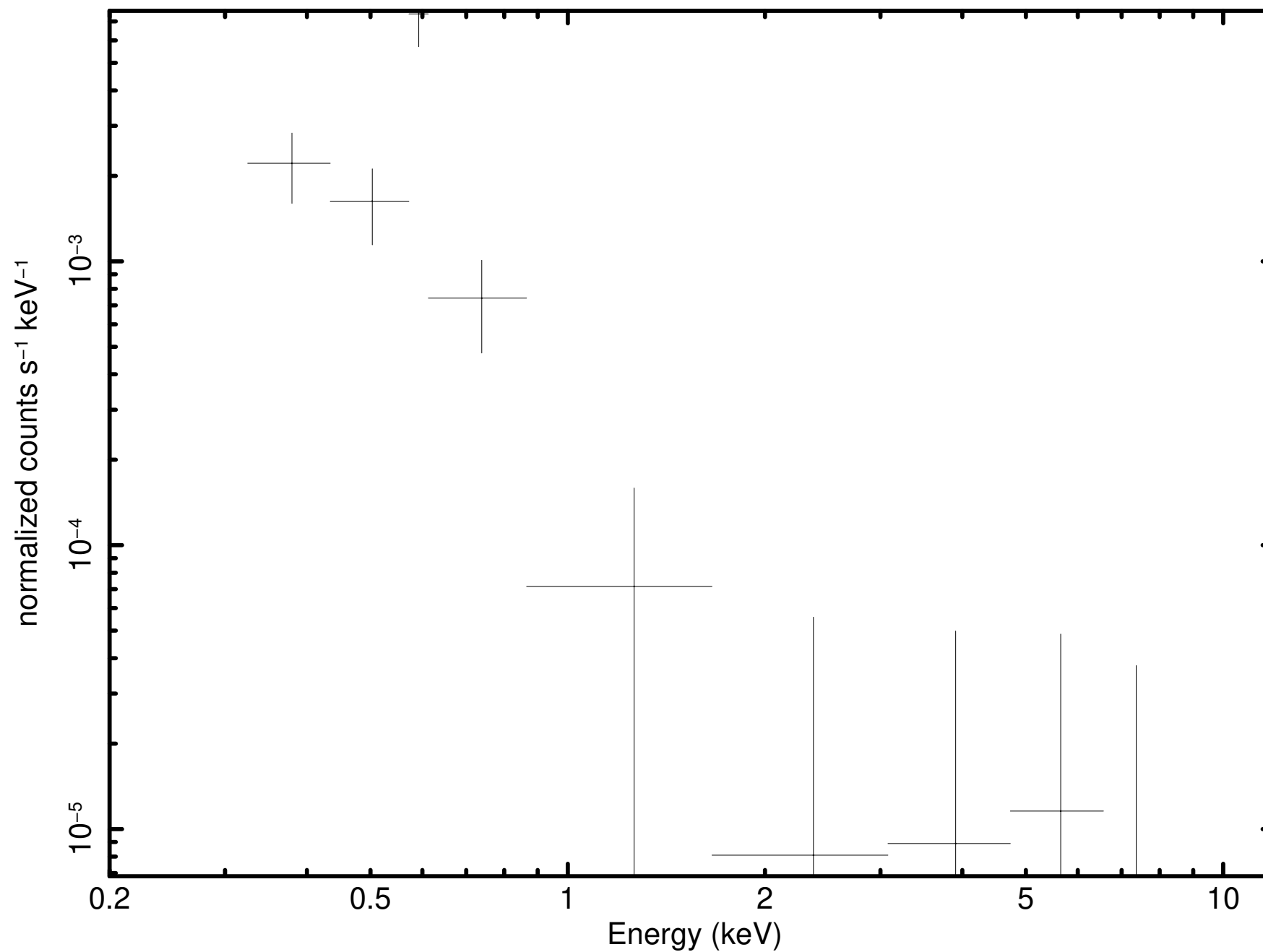
Source 76 minus background (P0931790101PNS003SRSPEC004C)
