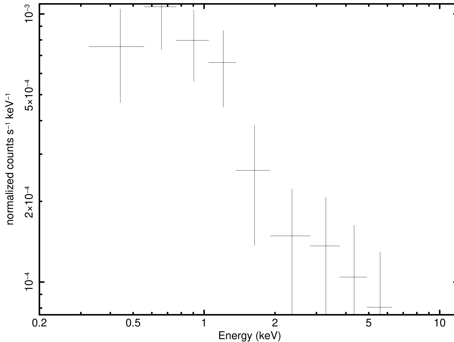
Source 77 minus background (P0931790101PNS003SRSPEC004D)
